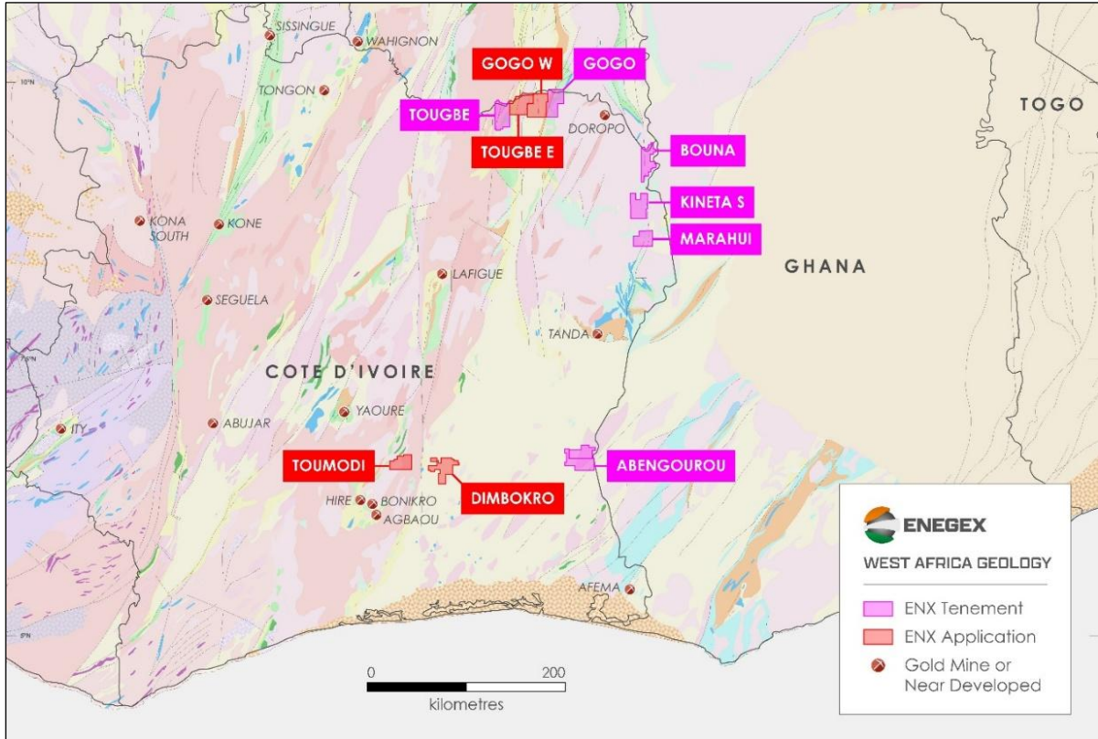
Figure 6: Birimian Belts in West Africa, showing EneSEX's ground position in Côte d'Ivoire including the Gogo-Tougbe permit group in the northern part of the country.
