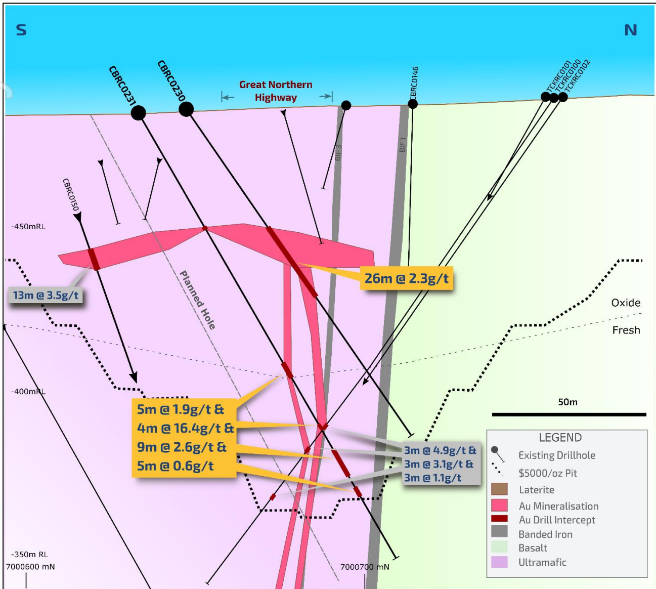
Figure 4 - Cross section through CBRC0230 and CBRC0231. Recent results in the yellow box. TCRRC0100 is off section.
