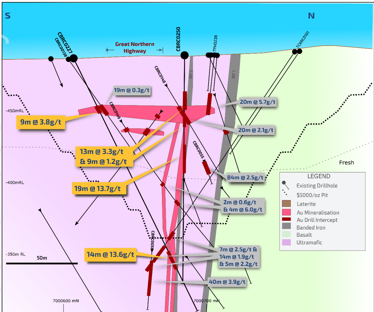
Figure 3 - Highway Cross Section through Hole CBRC0227 and CBRC0250 showing strong geological continuity and thick high grade oxide mineralisation. Previous holes CBRC0056 and TCKRC0101 are on the margins of the cross section.
