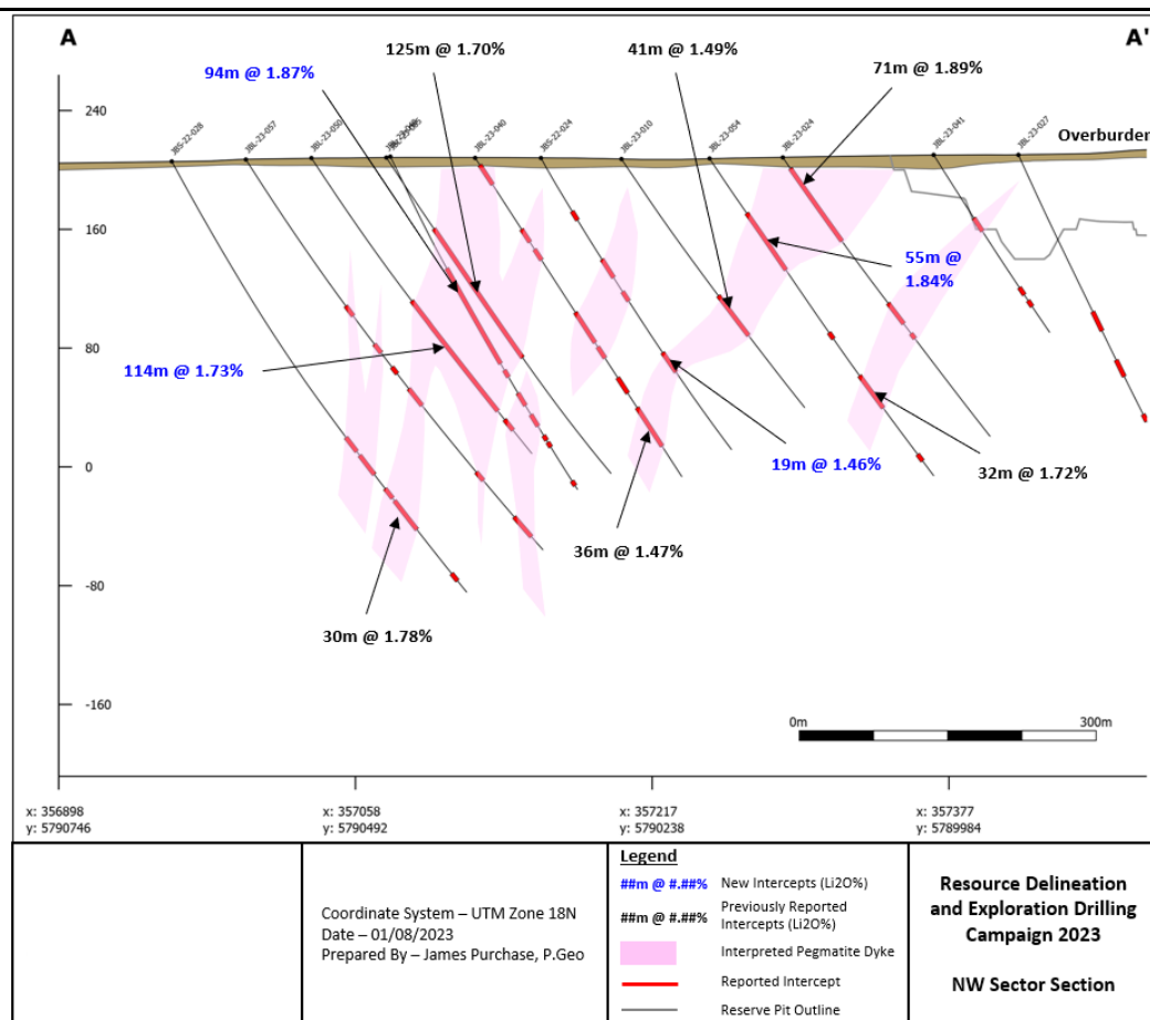
Figure 43 Galaxy section view of the northwest sector (looking northeast)
