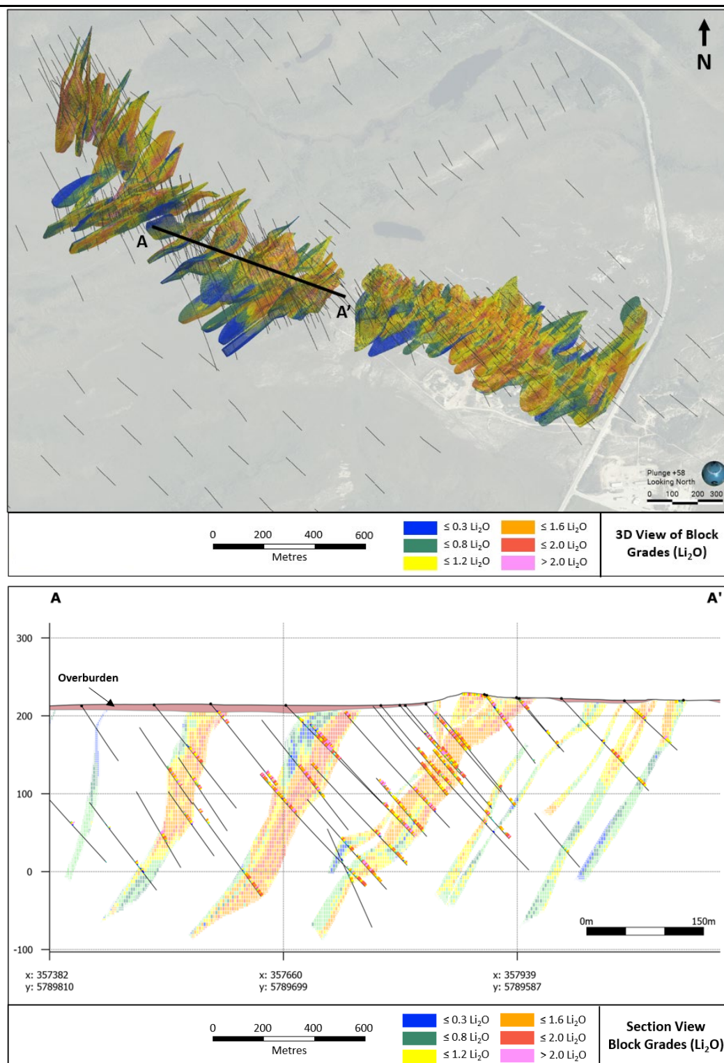
Figure 44 Galaxy isometric and section view (looking north) of Li 2 O block grades
