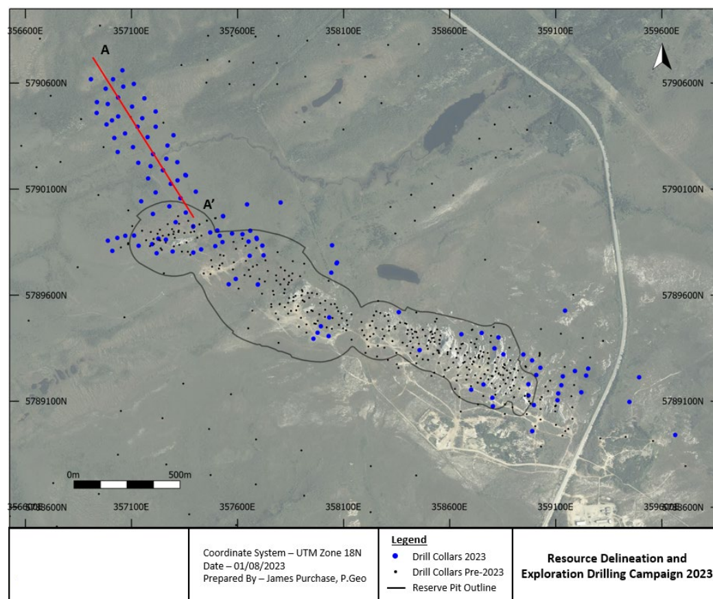
Figure 39 Galaxy plan view showing drill collars
