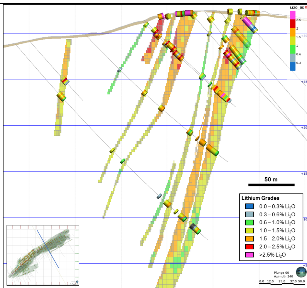
Figure 35 Whabouchi composite versus block grades – section 2 view looking southwest (UTM grid)
