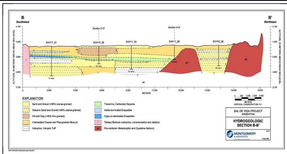
Figure 21 Sal de Vida hydrogeological cross section B-B'
