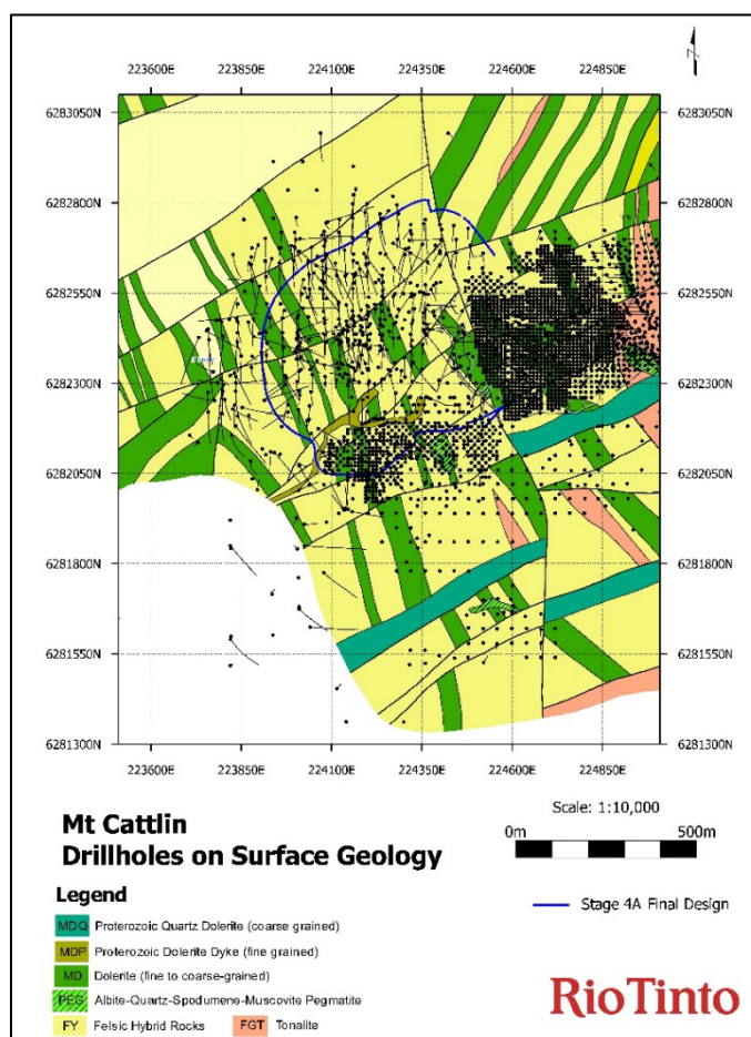
Mt Cattlin drillhole collars on pre-mining surface geology
