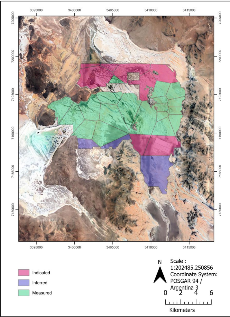
Figure 24 Sal de Vida Mineral Resources polygons
