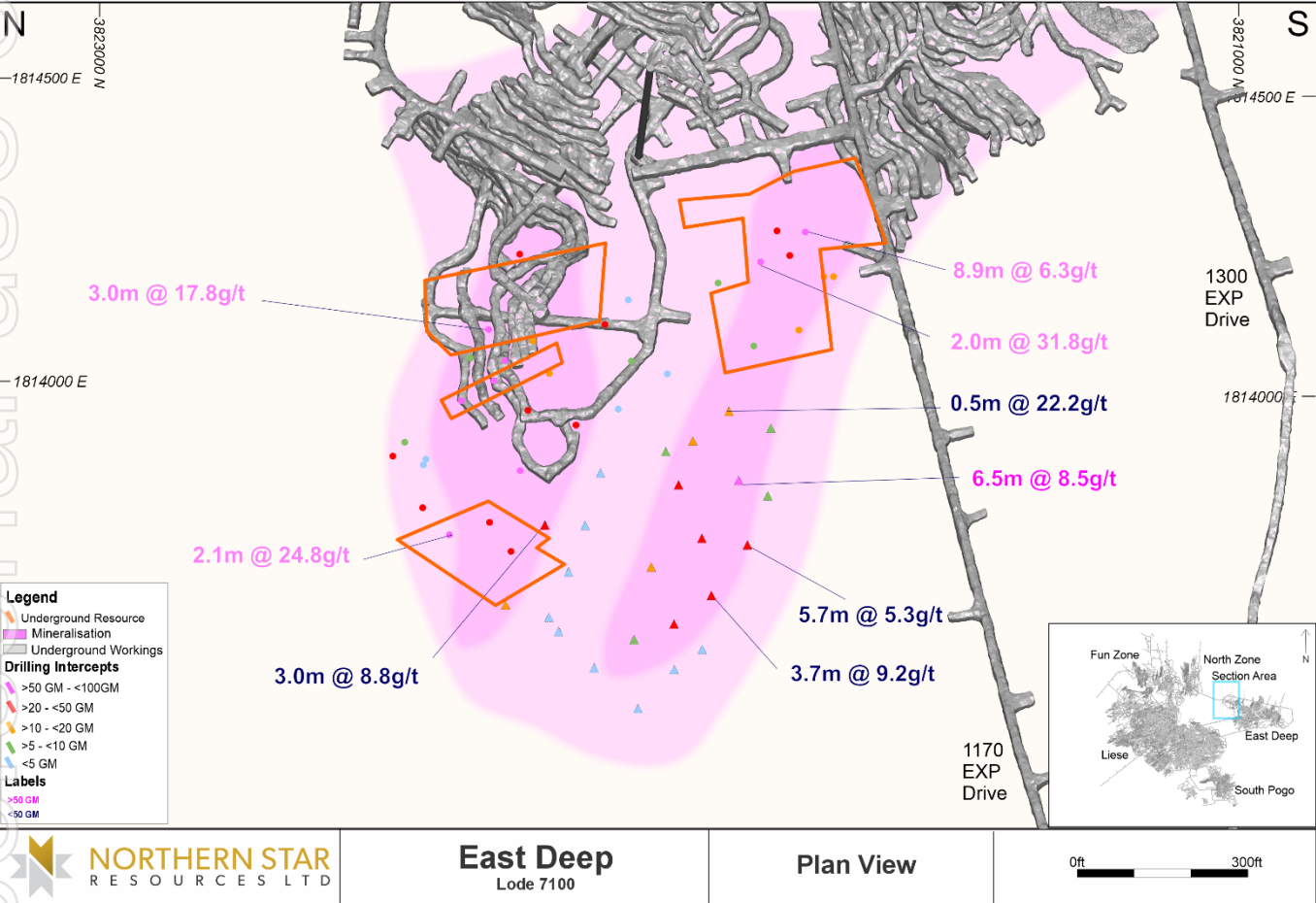
Figure 14 – East Deep Plan View and New Drill Results
