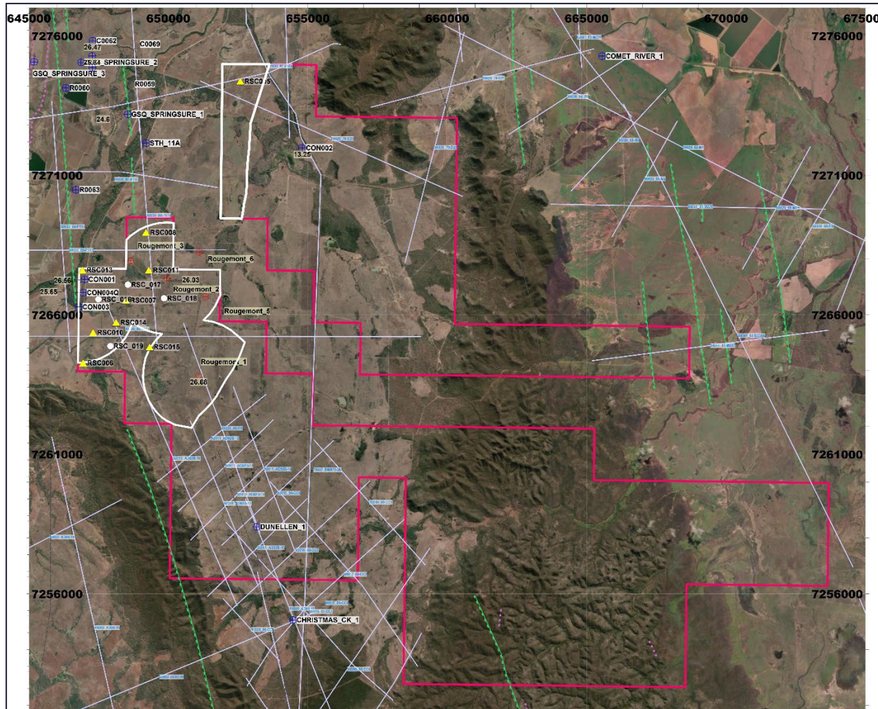
Figure A2-1: Location of 2025-2026 Planned Drilling (Yellow Triangles)
