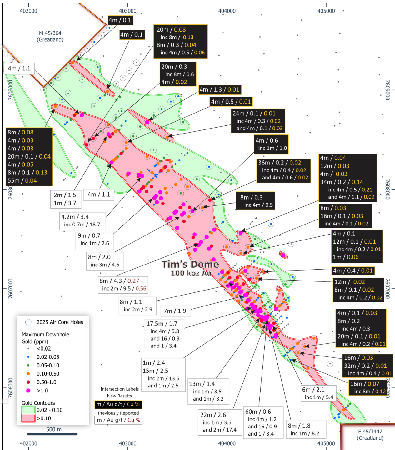
Figure 13: Map showing the Tim's Dome area, including Mineral Resource, and contoured maximum down-hole gold drill results. NB: Refer to Figure 9 for location information and GDA2020 / MGA Zone 51 co-ordinates, 1km grid.
