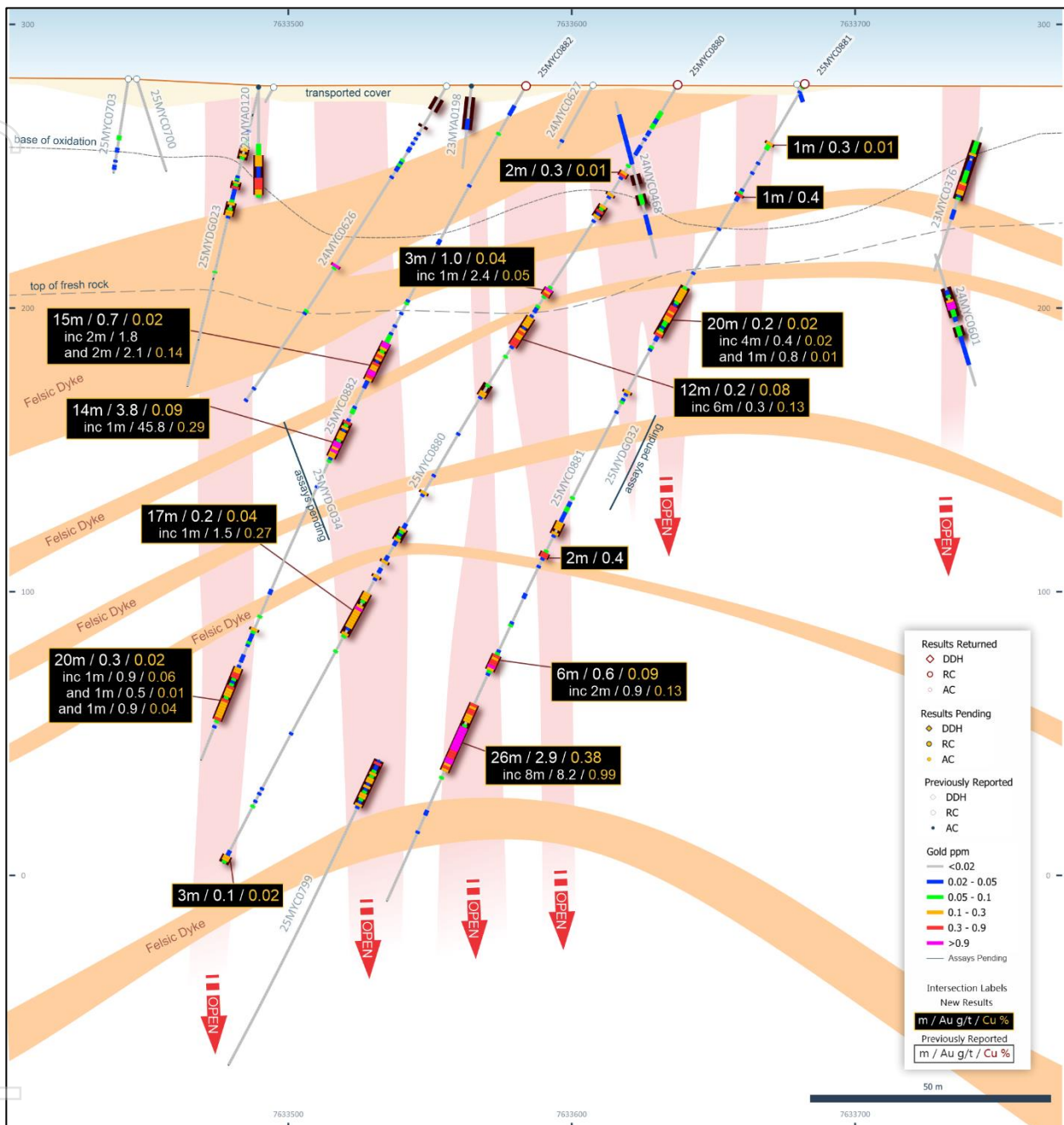
Figure 5: Fiama deposit GDA N-S cross-section 424,080 mE: Showing drill hole gold-copper drill intercepts including 25MYC0881 which extends high-grade gold mineralisation 110m down dip. The Fiama deposit remains open down dip for multiple zones of mineralisation. NB: Refer to Figures 2 to 4 and 8 for location information and 100m grid, looking toward 270° GDA2020 / MGA Zone 51 Grid.
