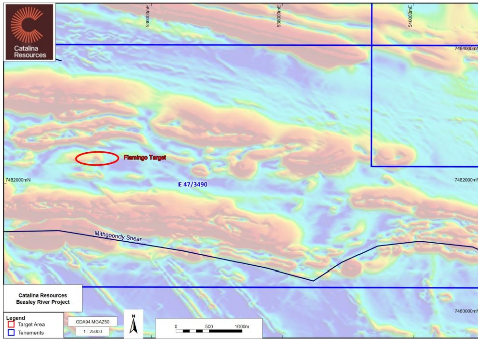
Figure 3. Rocklea map sheet overlay on TMI magnetic image showing the Flamingo target coinciding with the termination of a mapped structural trend and a NW-SW trending dolerite.
