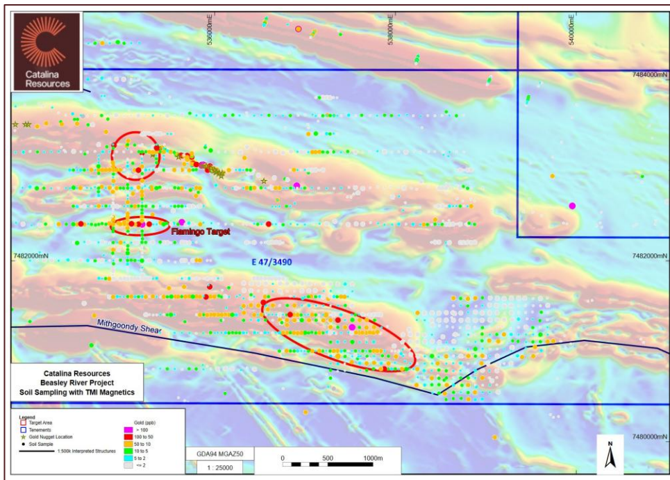
Figure 4. Anomalous Au, Cu, and As soil sample and magnetics coinciding with the structural trend north of the Mithgoody Shear.
