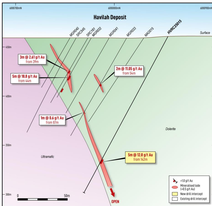
Figure 4: Cross Section looking west of drillhole HVRC25015, close to the Maninga Marley historic workings at the Havilah camp.
