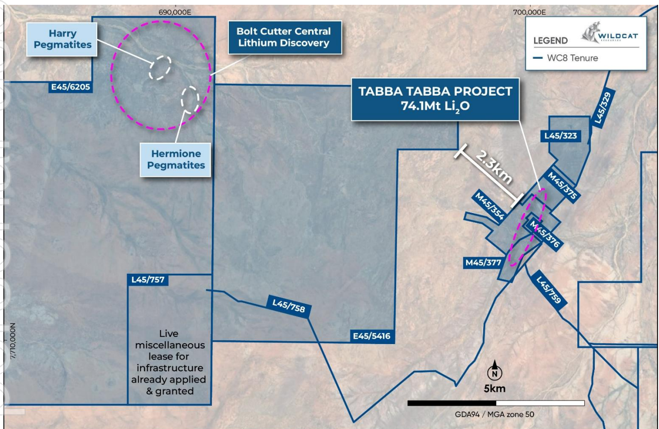
Figure 4: Location of the Bolt Cutter Central discovery relative to the Tabba Tabba Project, WA.
