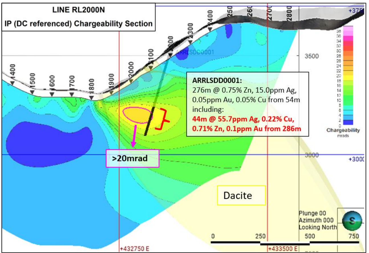
Figure 4: 2D IP chargeability section on line 2000 within BRX tenure (refer to Figure 2 for section location on plan view). Note the purple outline indicating a chargeability anomaly of >20mrad.
