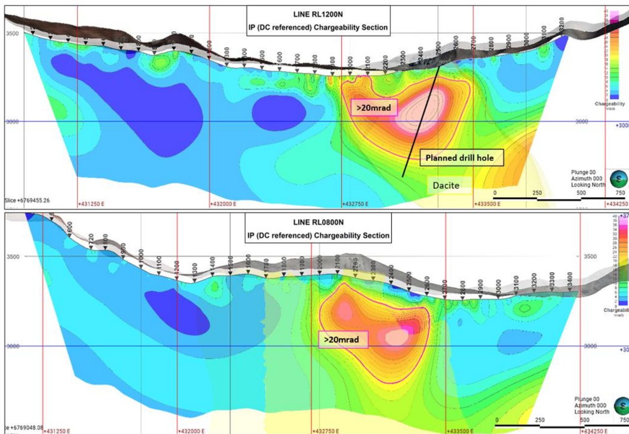
Figure 6: 2D IP chargeability section on line 1200 (top image) and 0800 (bottom image; refer to Figure 2 for section location on plan view). Note the purple outline indicating a chargeability anomaly of >20mrad and its marked increase in size and intensity compared to line 2000.
