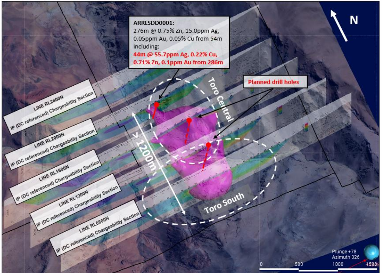
Figure 3: Oblique Plan view of the interpolated 3D volume of the chargeability anomaly from the 2D IP chargeability sections. Note the purple outline indicating a chargeability anomaly of >20mrad and its marked increase in size and intensity to the south compared to line 2000.
