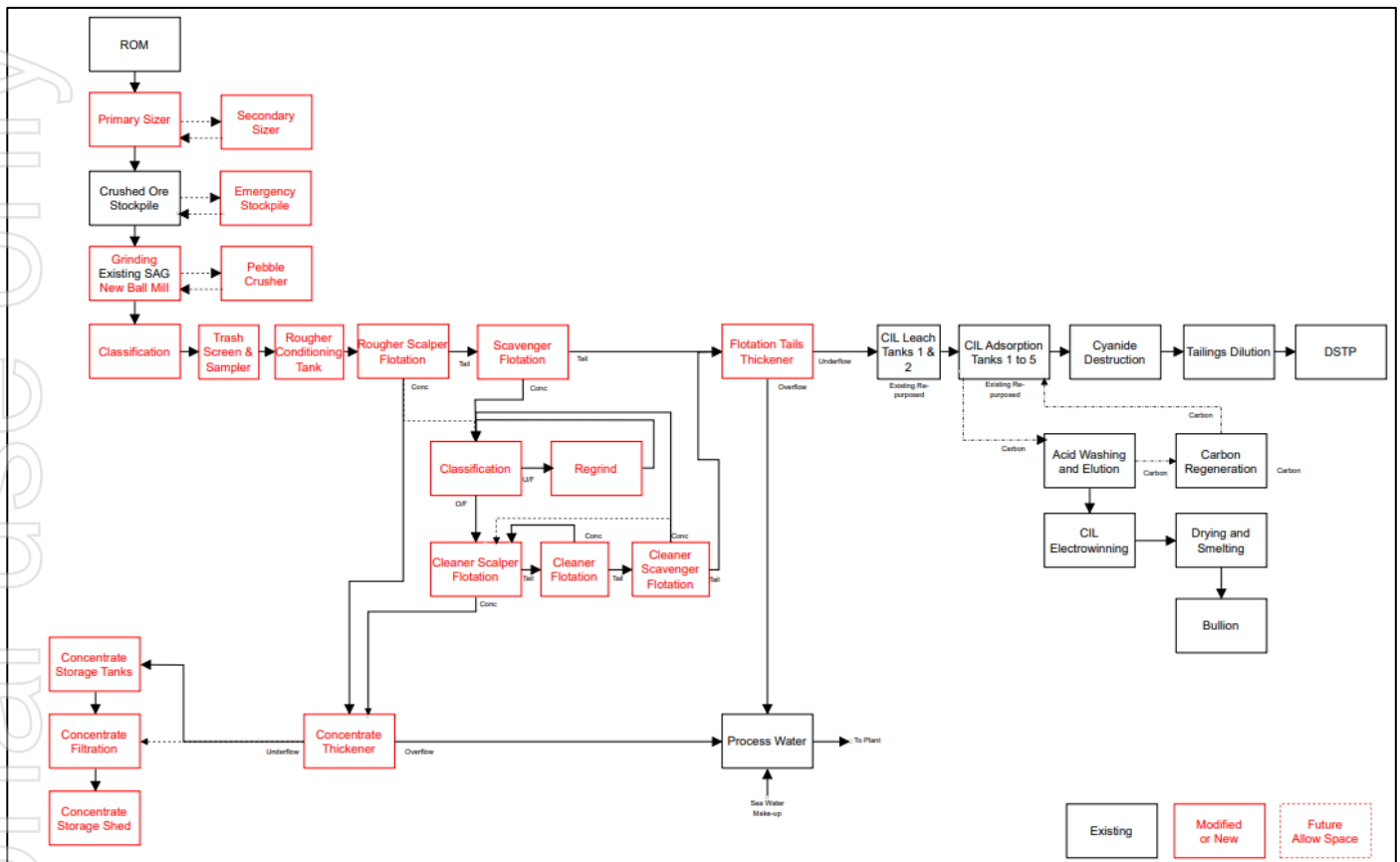
Figure 7: Saleable Concentrate Flowsheet – Block Flow Diagram
