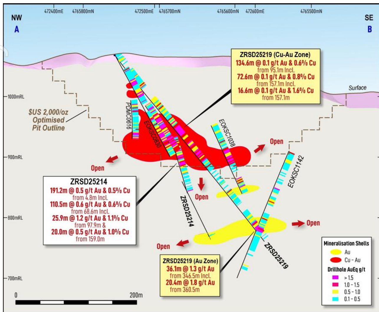
Figure 3. Copper Canyon cross-section view along A-B, showing results for ZRSD25219 in relation to previously reported drill intercepts. 3
