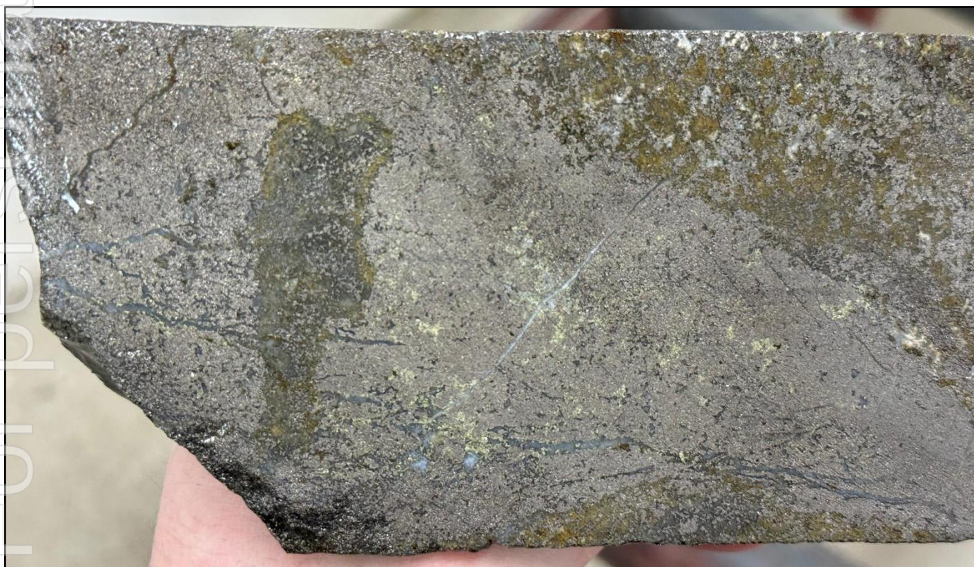
Figure 5. Core photograph from sample interval 48.2m to 49.1m in ZRSD25223, showing replacement style mineralisation with semi-massive pyrrhotite, chalcopyrite and pyrite assaying 1.8g/t Au, 2.1% Cu, 10.6g/t Ag (5.8g/t AuEq).
