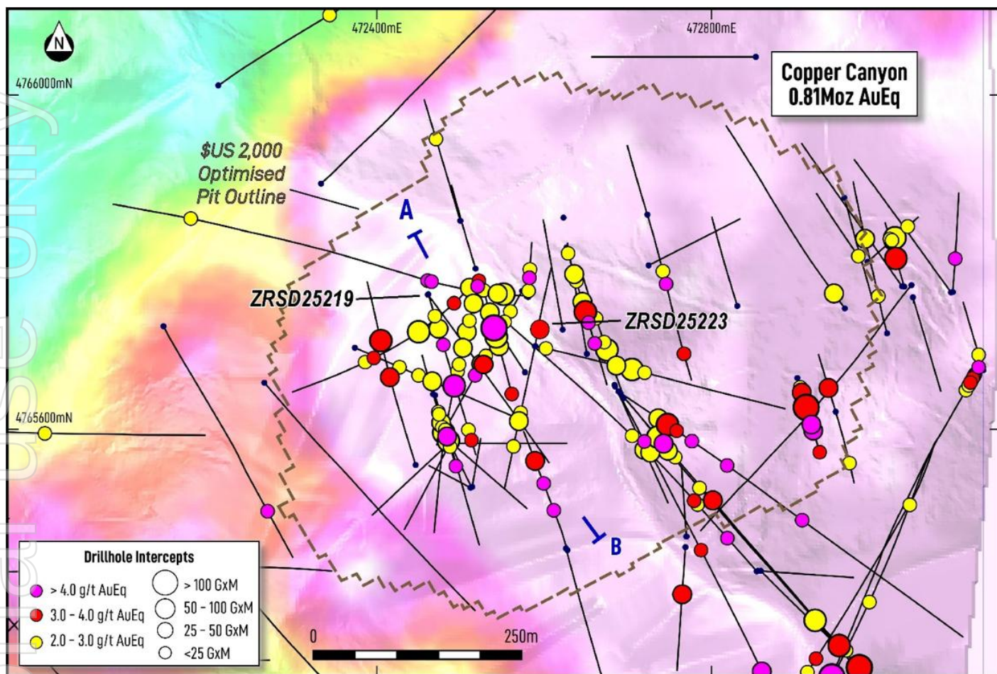
Figure 2. Plan view map of the Copper Canyon Deposit, showing drill-holes reported in this announcement, drill-hole intercepts, gold-arsenic soil geochemical response, optimised (@ US$2,000/oz) pit outline and section line for the Figure 3.
