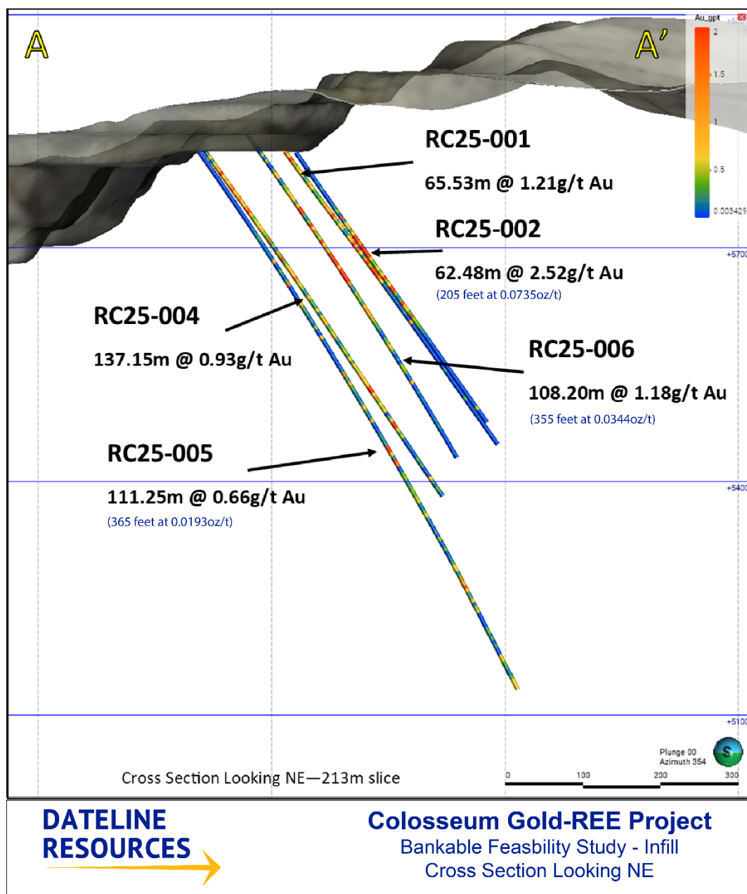
Figure 2: Cross-section of the Colosseum deposit illustrating the existing open pit outline and gold intercepts
