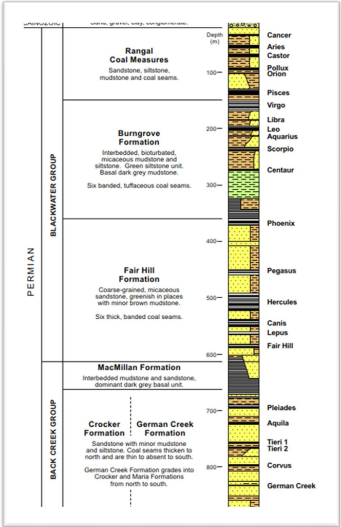
Figure 2 Generalised stratigraphy of Blackwater
