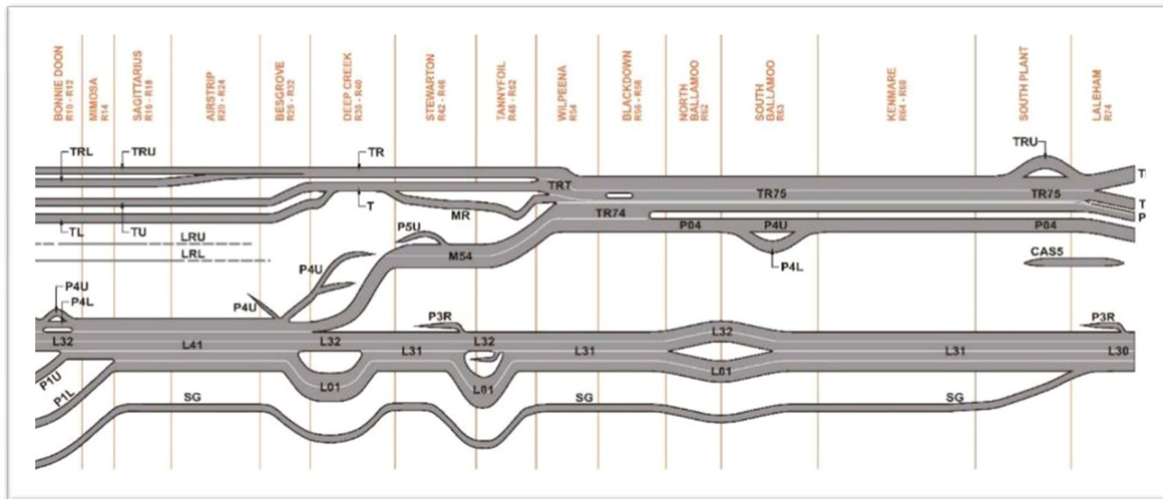
Figure 3 Blackwater seam stratigraphy
