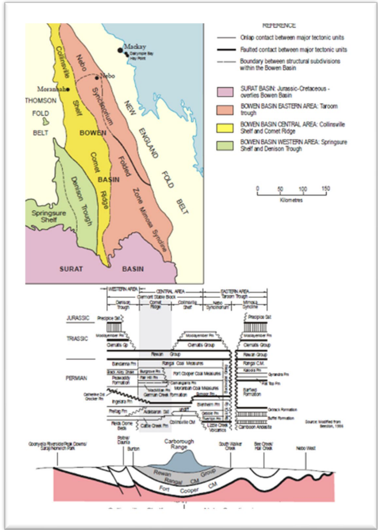
Figure 1 Tectonic troughs, shelves and stratigraphy of the Bowen Basin
