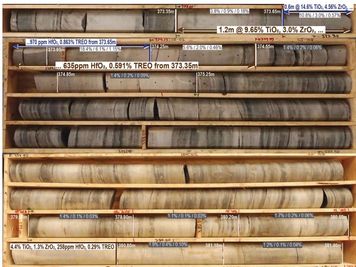
Black: TiO 2 % / ZrO 2 % / TREO% (individual sample) Brown: 2% TiO 2 cut-off Blue: 8% TiO 2 cut-off Figure 4 – SOR-02 diamond drill core photos showing individual sample assays and weighted average assay highlights.
