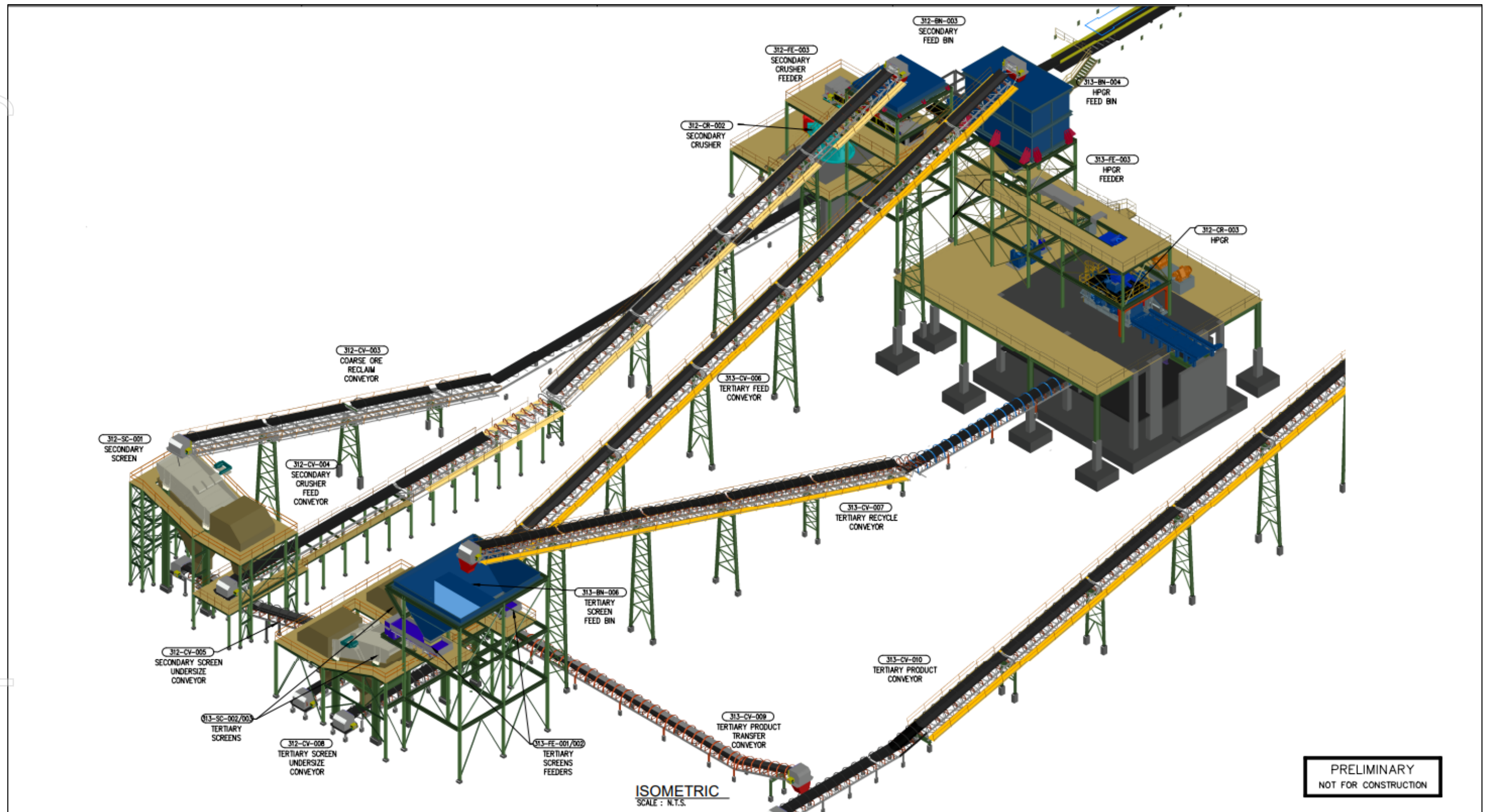
Figure 5.3: Secondary and Tertiary Plant Isometric Image.
