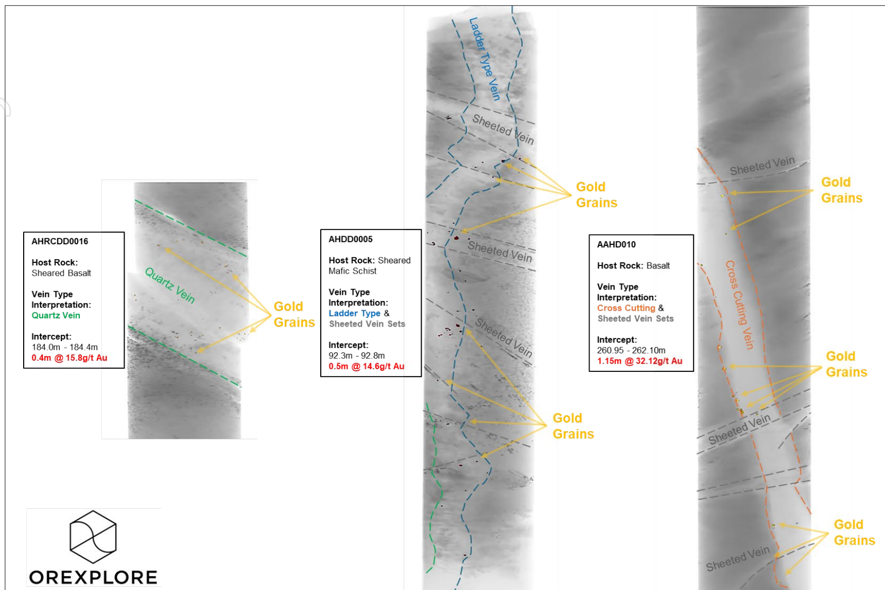
Figure 4.1: Apollo Hill Quartz Veins and Gold Department in Fresh Basalt NQ2 Diamond Drill Core (Images by Orexplore).
