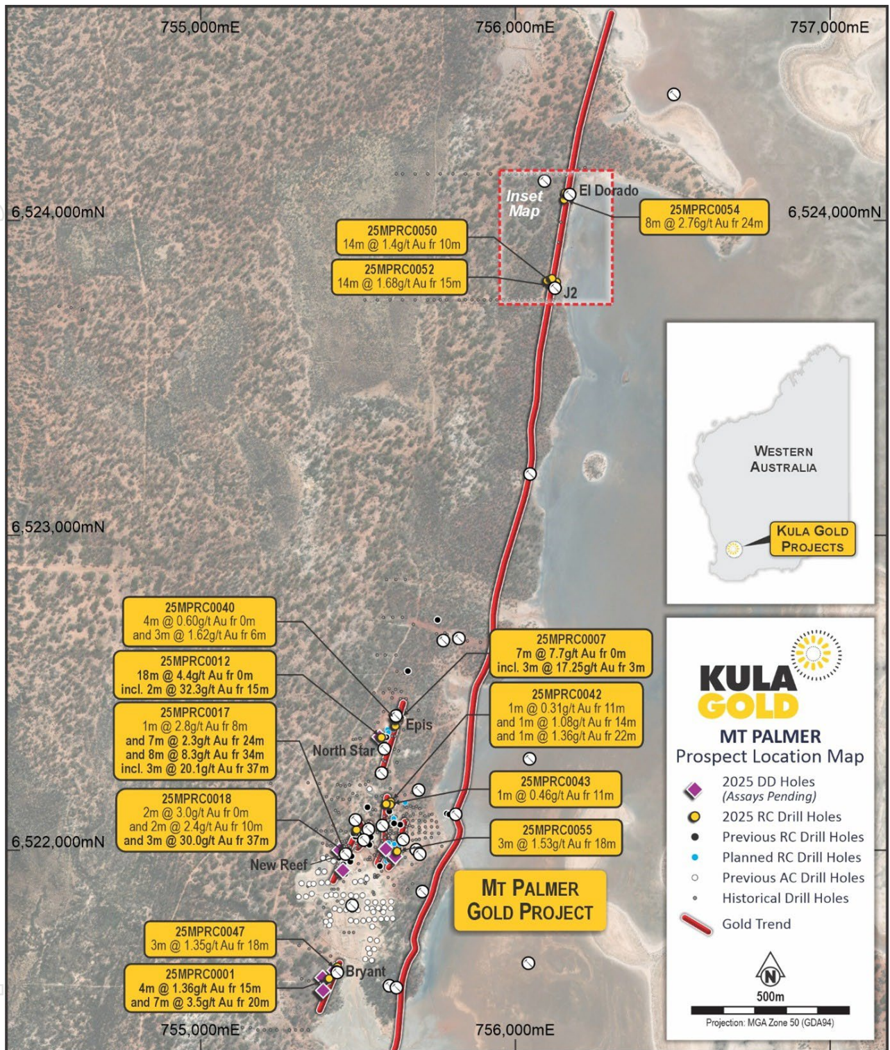
Figure 9: El Dorado trend over 3km strike shown in red with some of the promising drill results
