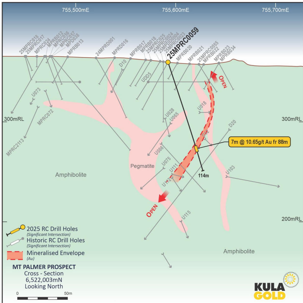
Figure 2: Cross Section for 25MPRC0059
