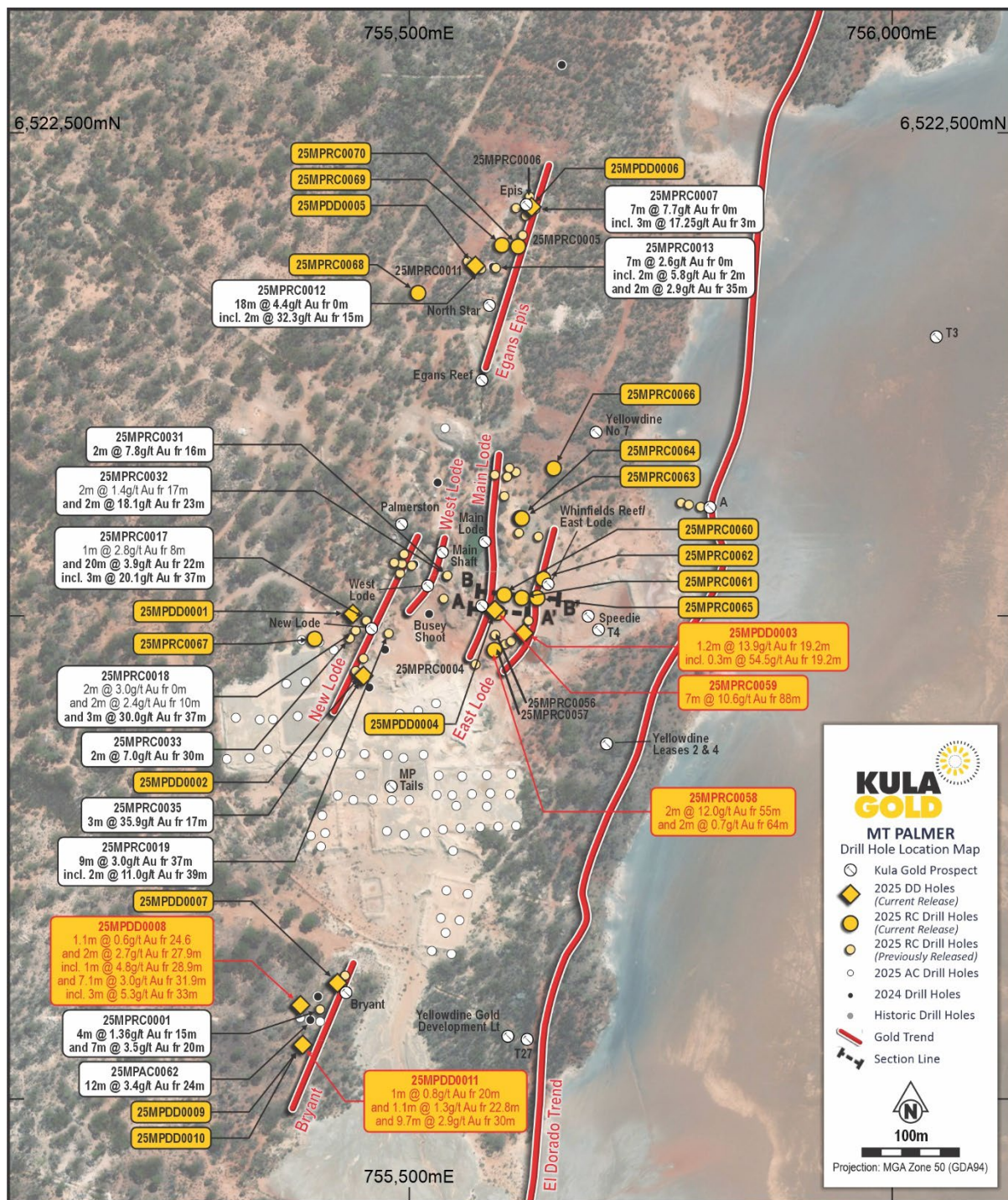
Figure 1: Kula's Mt Palmer Gold Project
