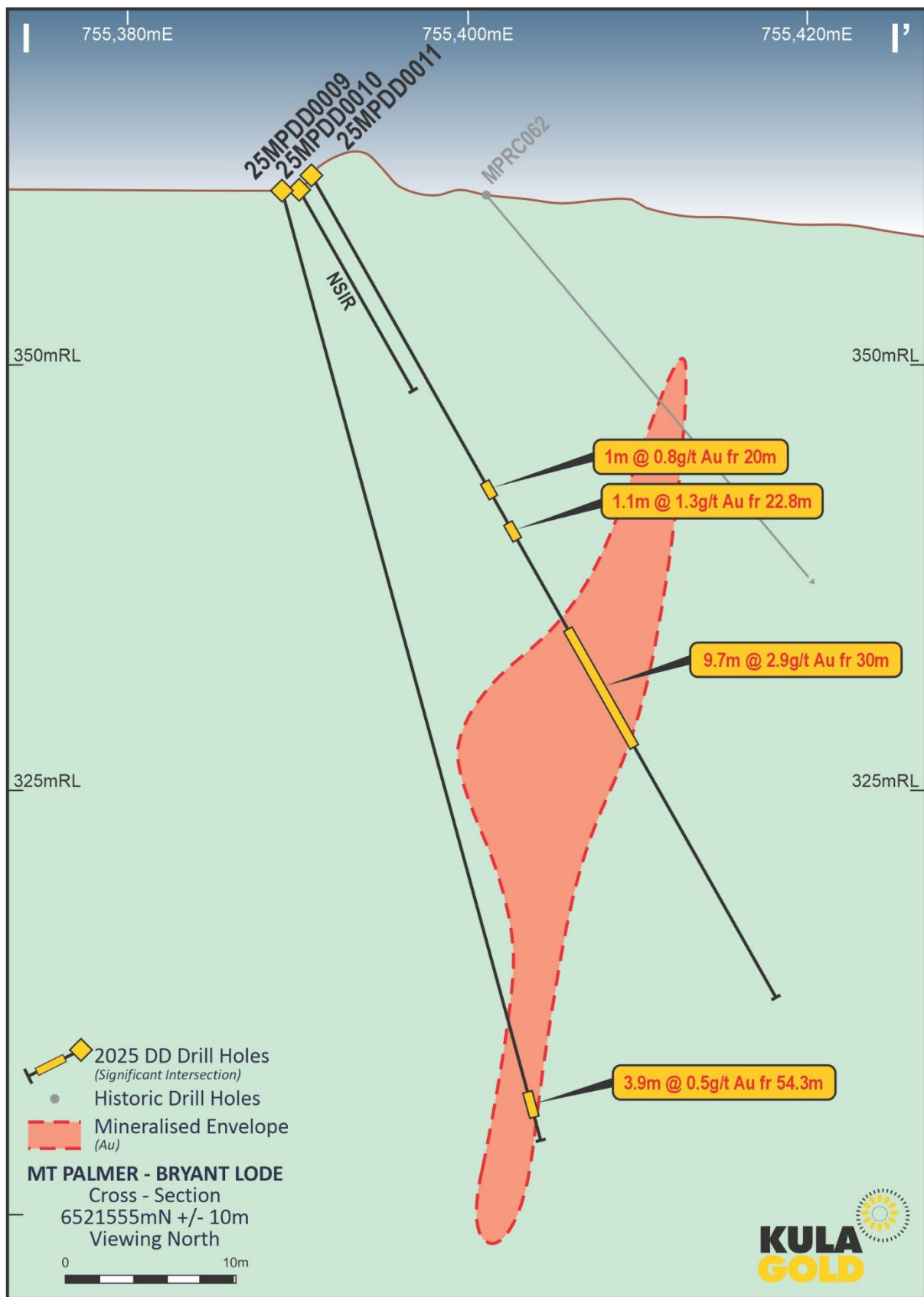
Figure 7: Cross Section for 25MPDD009, 10 and 11
