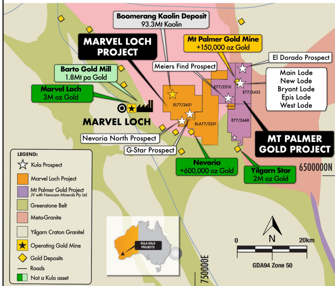
Figure 10: Kula's Marvel Loch Region Tenure
