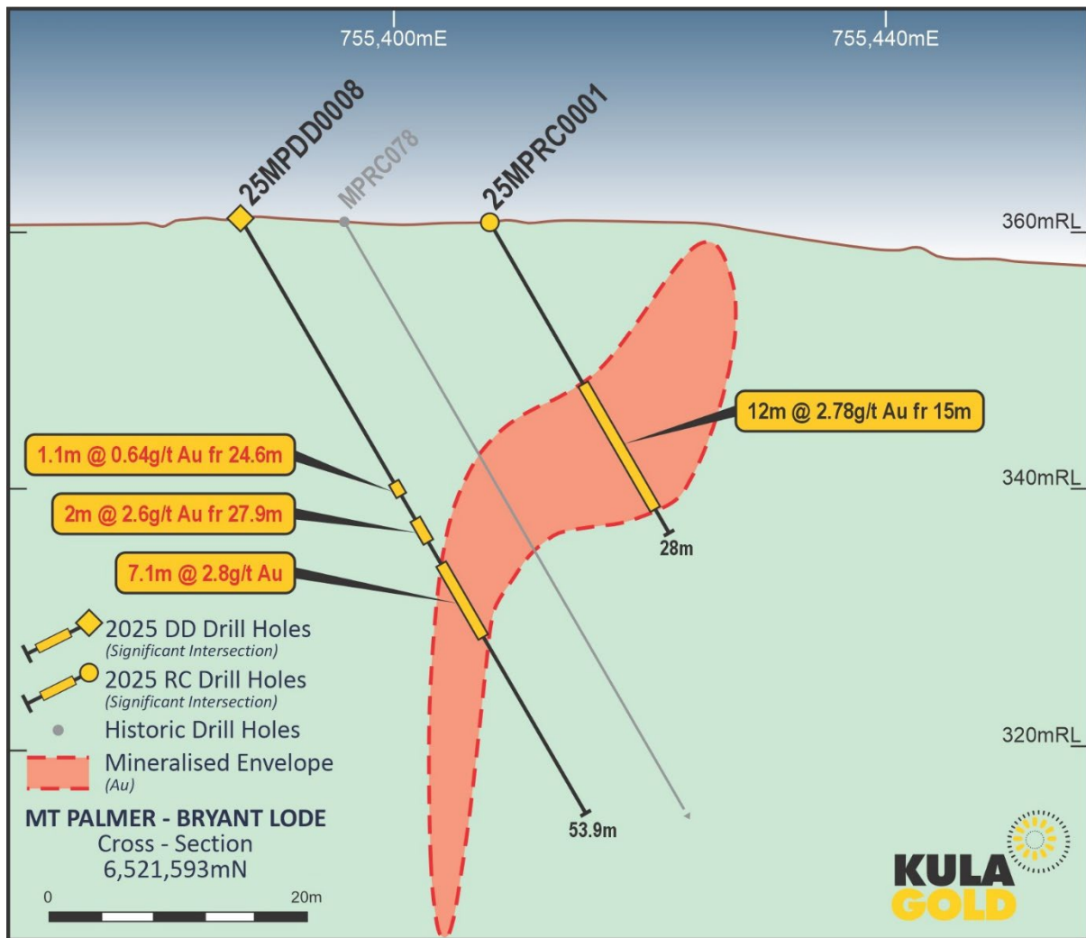
Figure 8: Cross Section for 25MPDD0008
