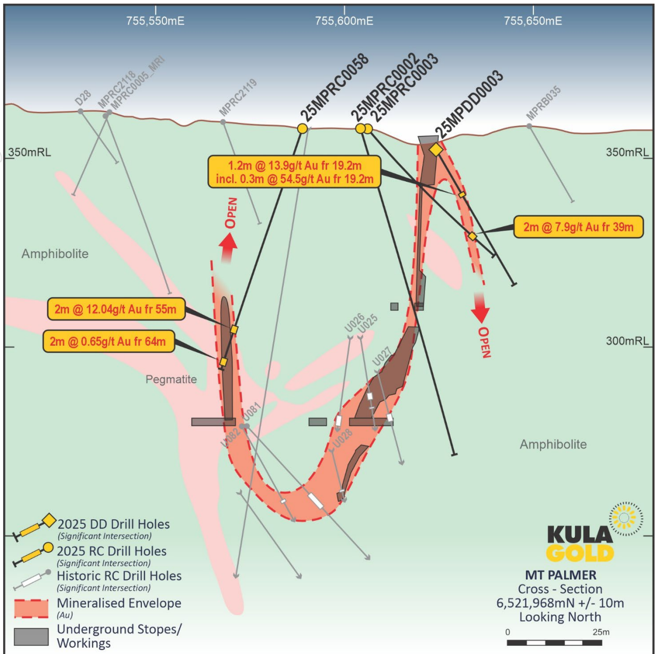
Figure 4: Cross Section for 25MPDD0003 and 25MPRC0058
