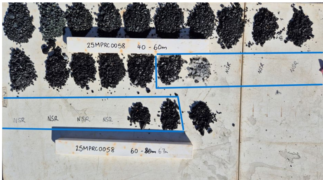
Figure 6: 25MPRC0058: starting from 55m assays show 2m @ 12.04g/t gold, then mined void for 7m (denoted as NSR in photo), then 2m @ 0.65g/t gold -giving a total zone of 11m
