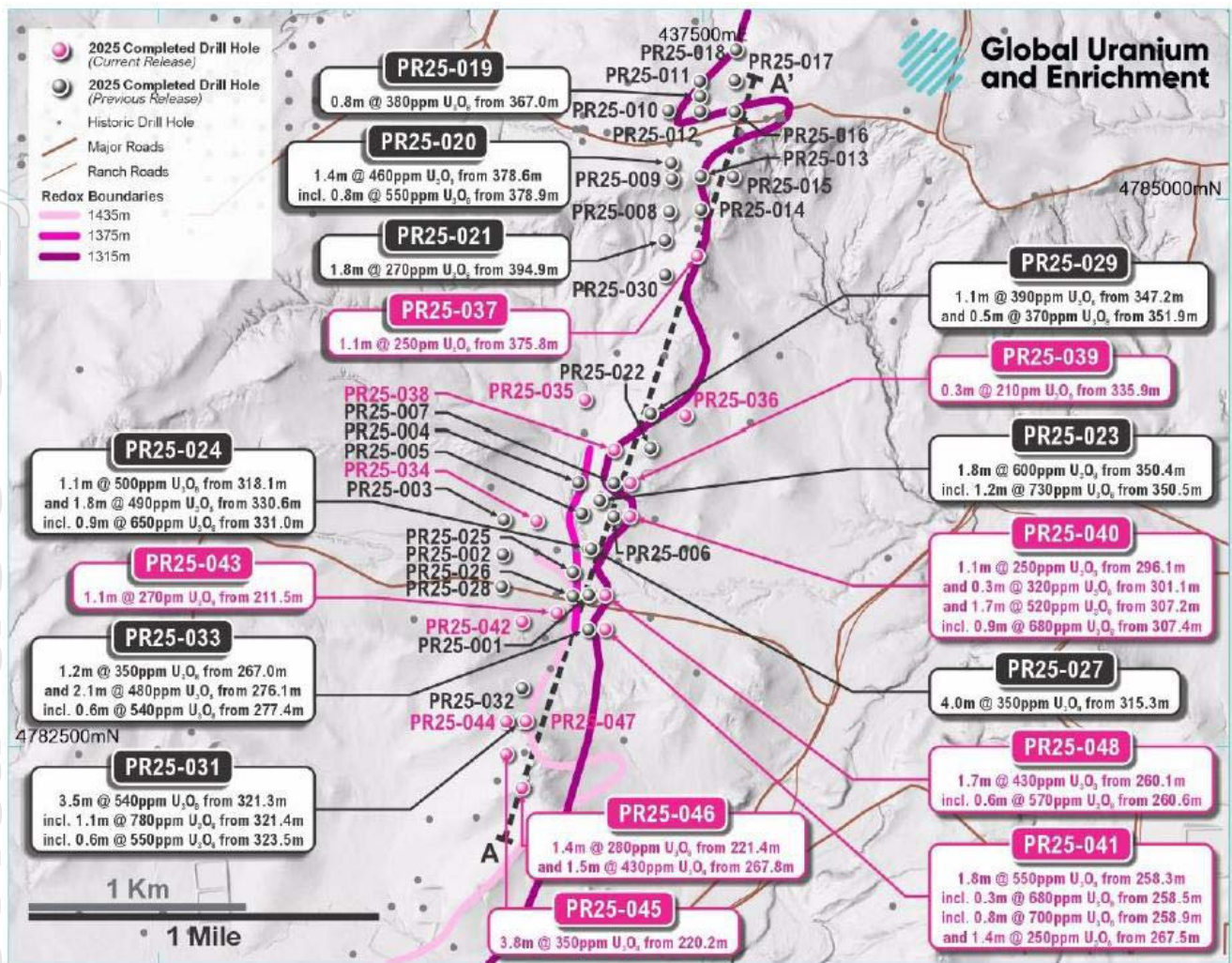
Figure 6: Detailed map showing the locations and results of recent holes drilled at the Pine Ridge Project.
