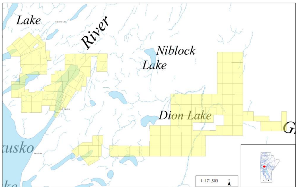
Figure 13 – Map showing the Snow Lake Lithium Project
