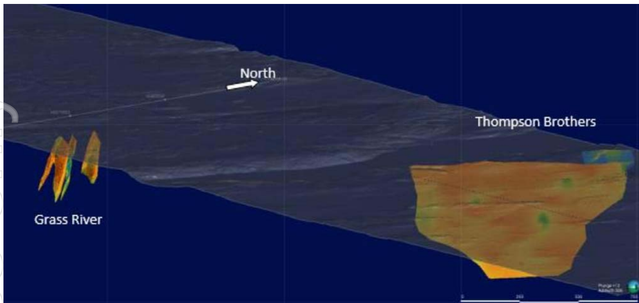
Figure 16: Isometric view of the block model of the TB and GR deposits coloured by LiO 2 grade
