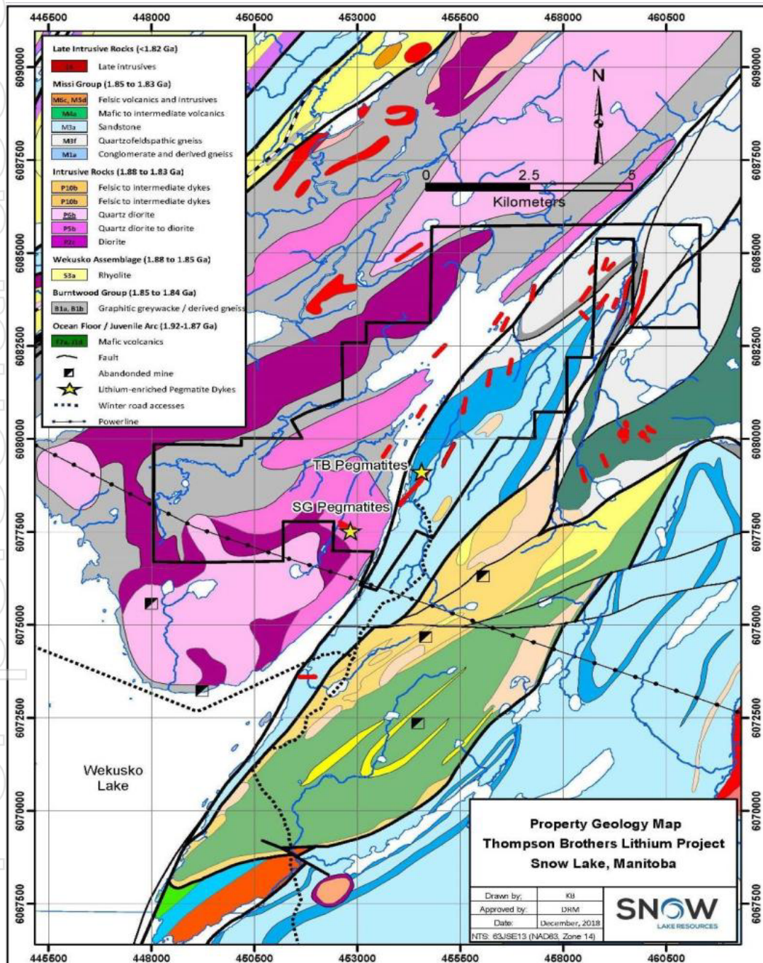
Figure 15: Geological Map of the Snow Lake Lithium Project
