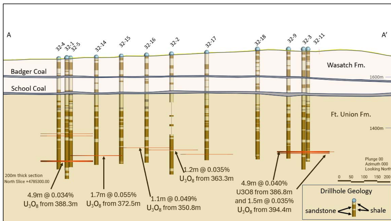
Figure 7 - Pine Ridge Uranium Project Cross Section on highest GT mineral intercepts.
