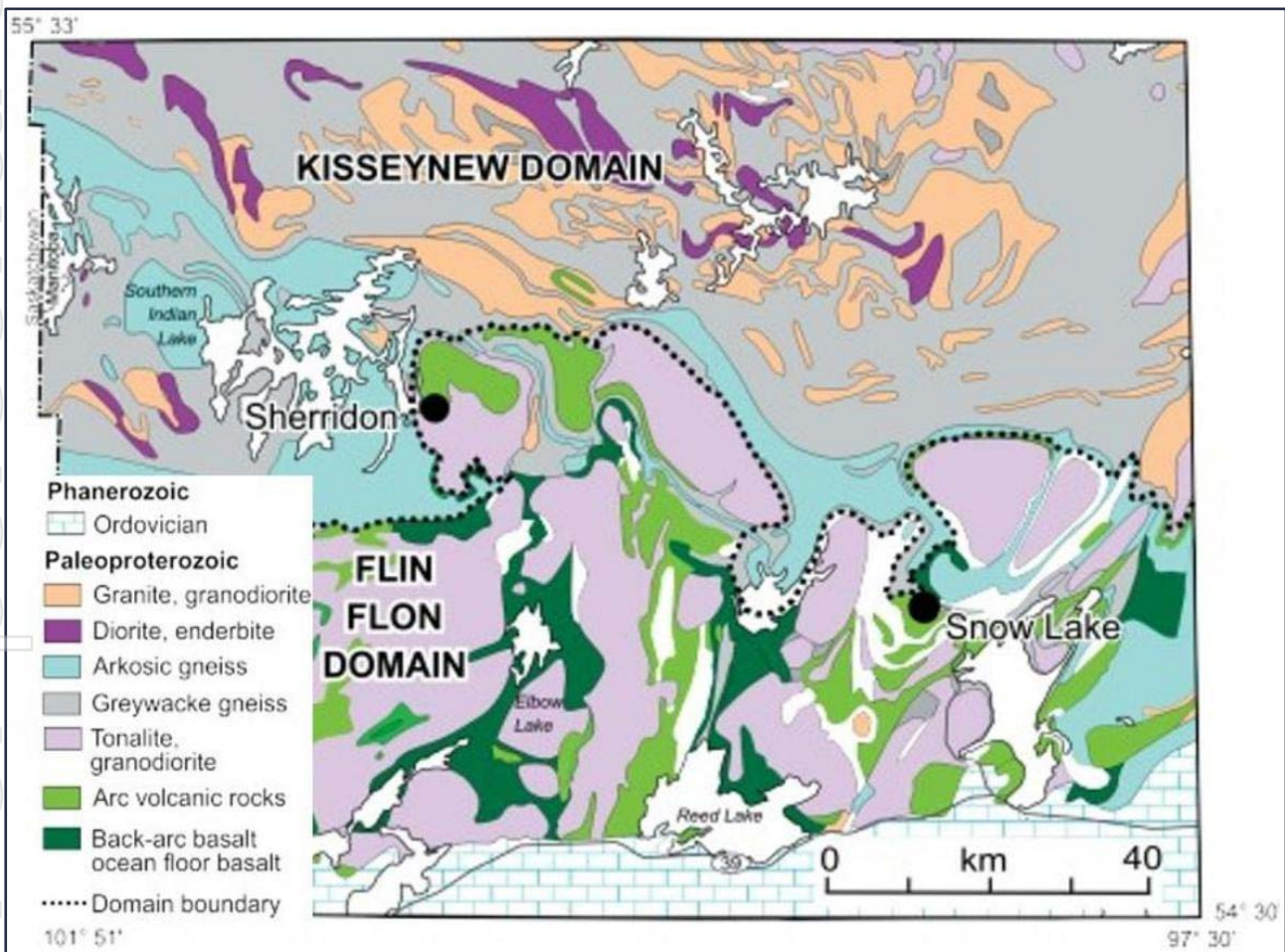
Figure 14: Geological setting of the Snow Lake Lithium Project
