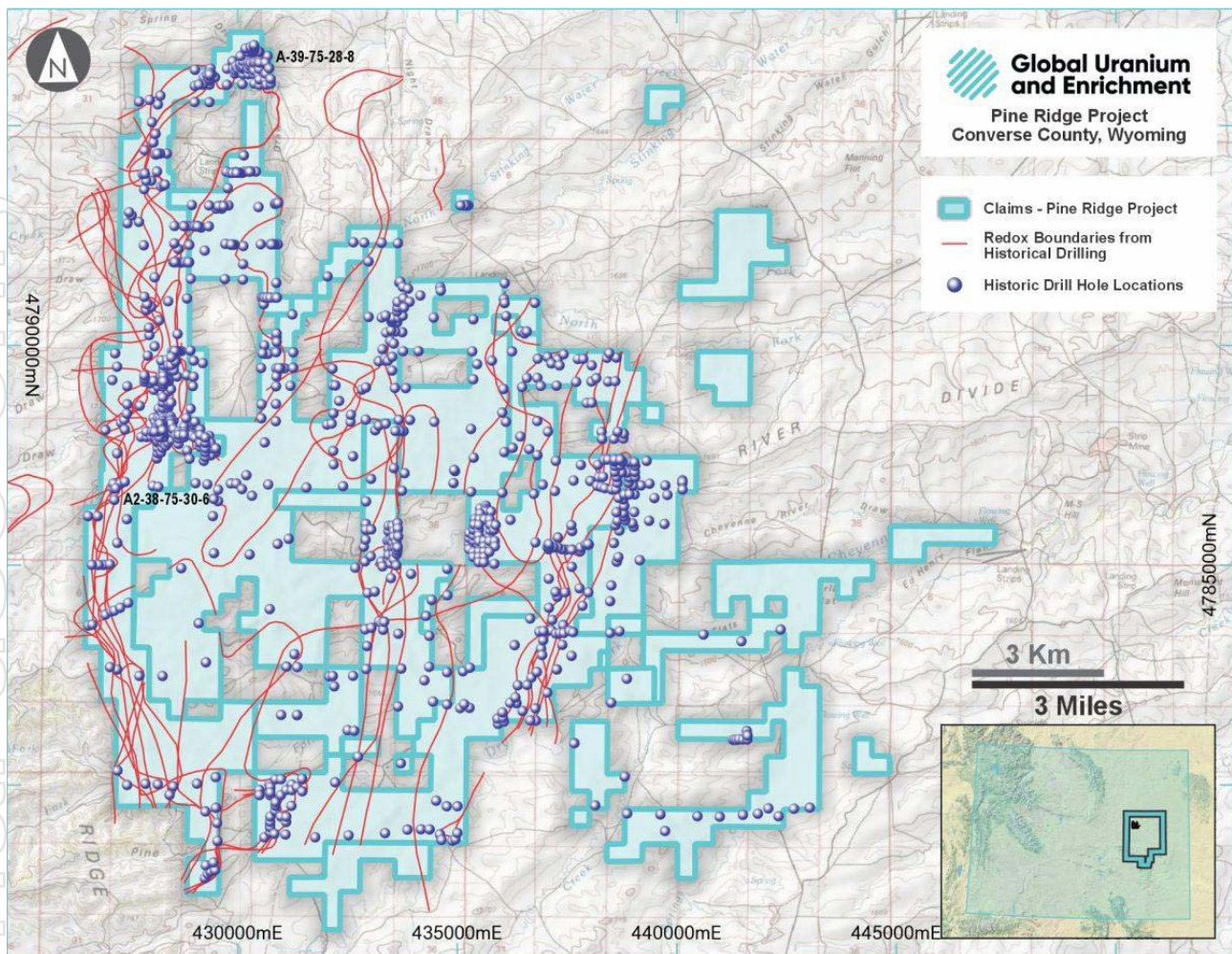
Figure 4: Pine Ridge Project Redox boundaries and historical drillhole positions
