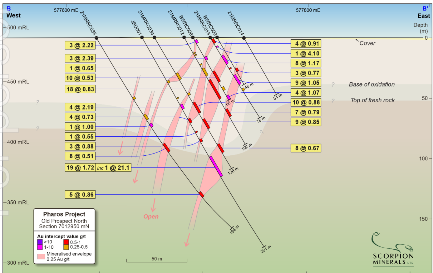
Figure 6: Old Prospect North Section B – B'
