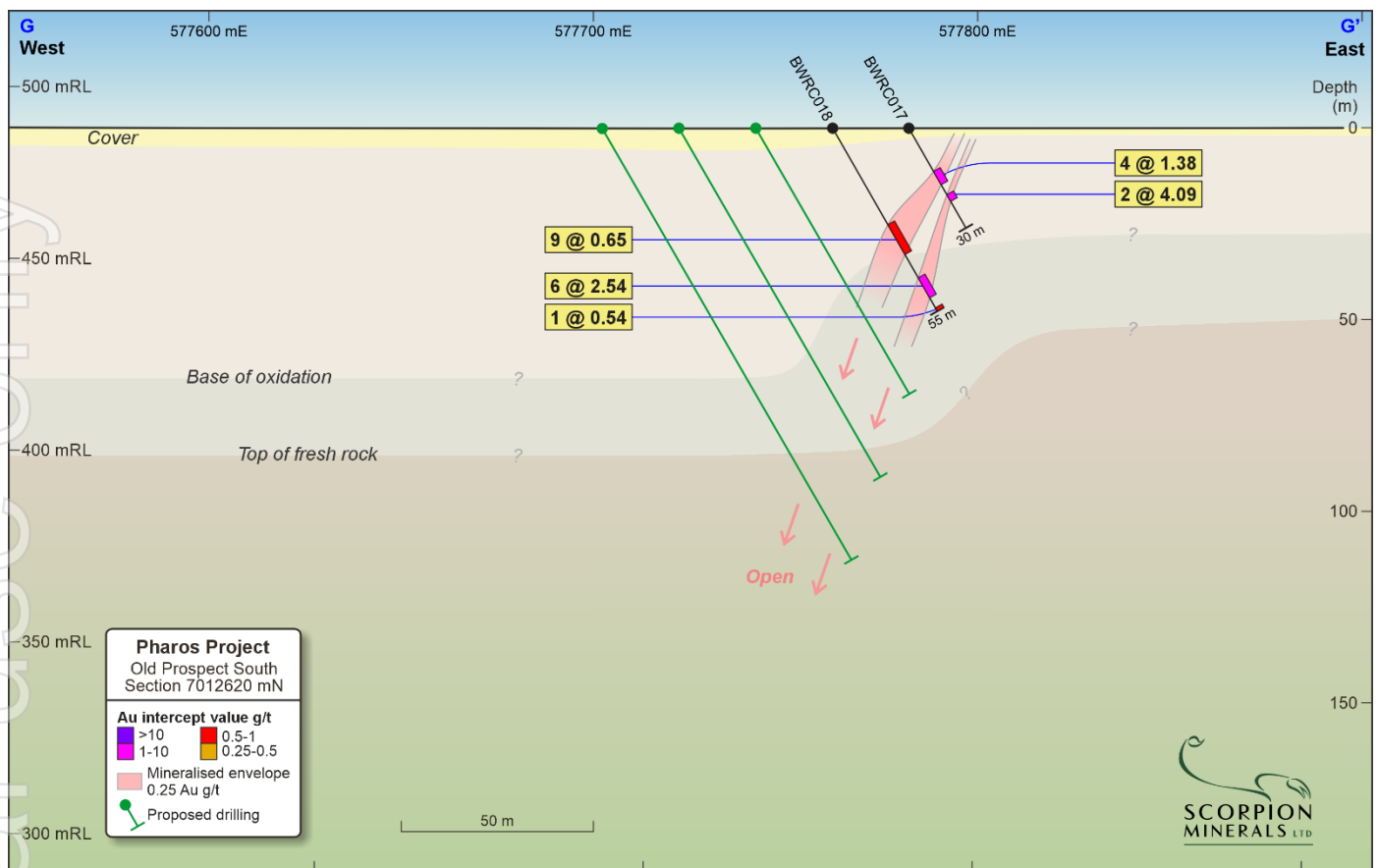
Figure 11: Old Prospect South Section G – G'
