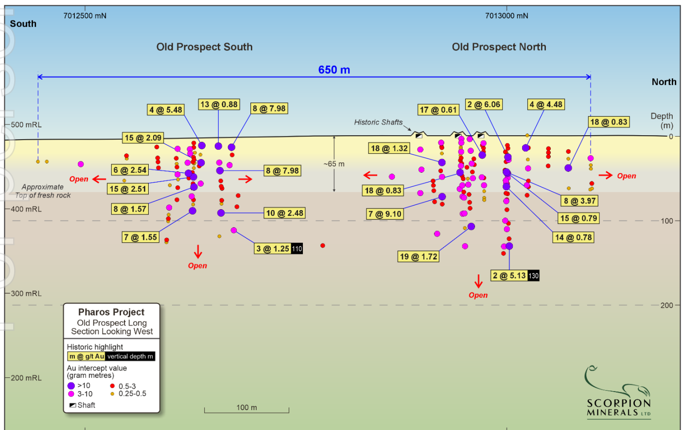
Figure 12: Old Prospect Long Section Looking West
