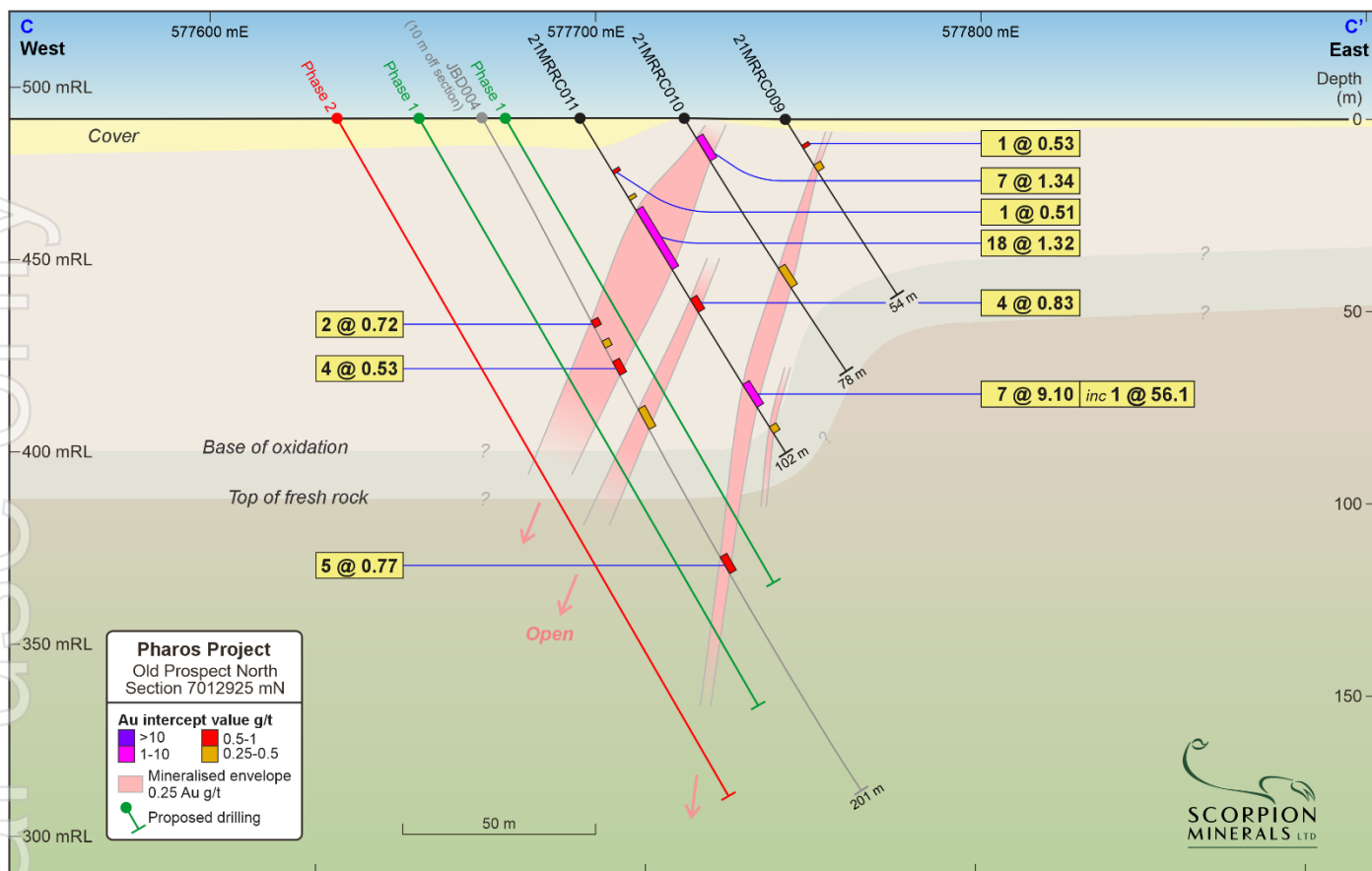
Figure 7: Old Prospect North Section C – C'
