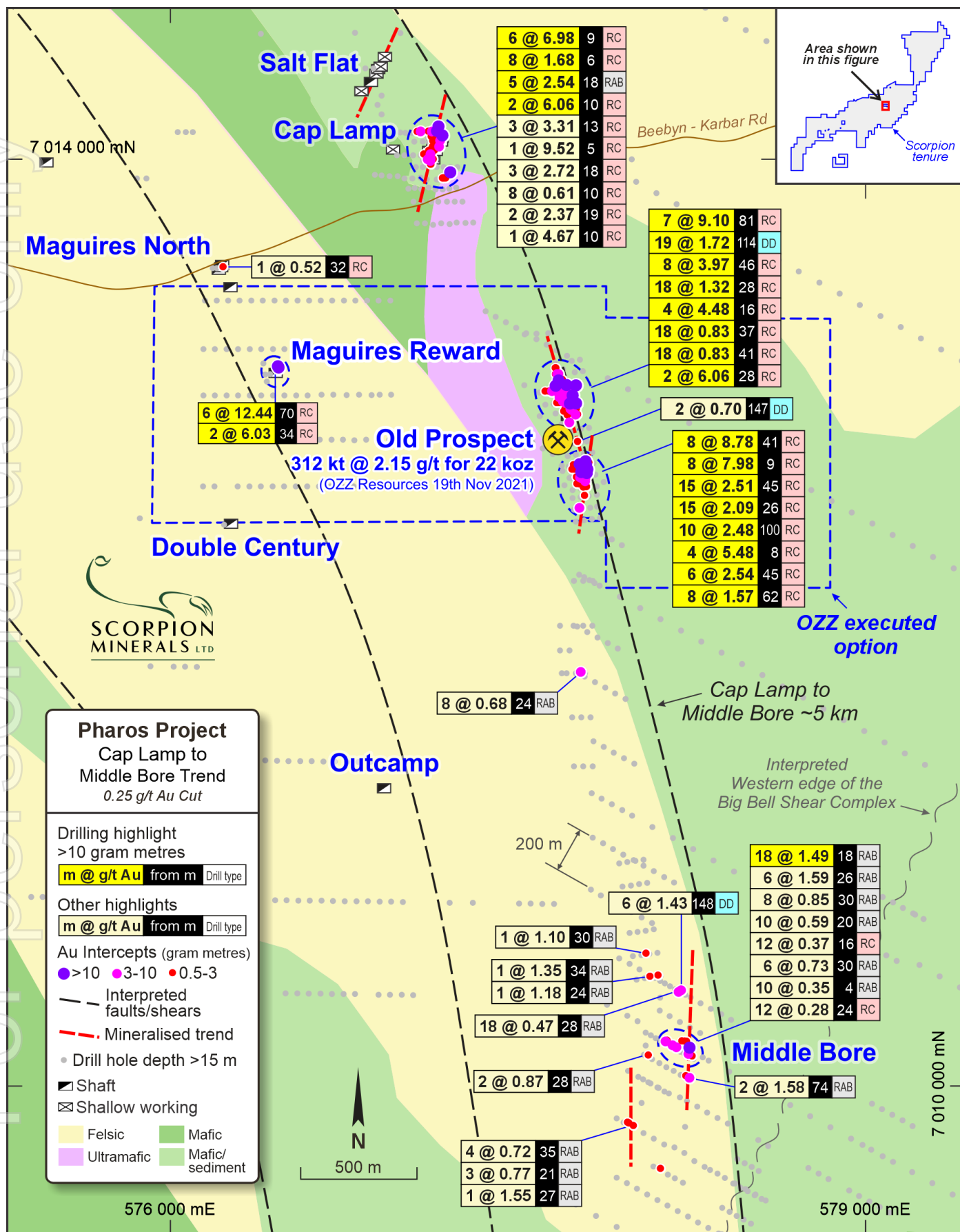
Figure 3: Cap Lamp to Middle Bore Overview highlighting Old Prospect RC drilling results within 5km long structural corridor
