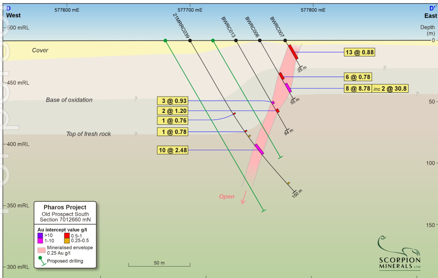
Figure 8: Old Prospect South Section D – D'
