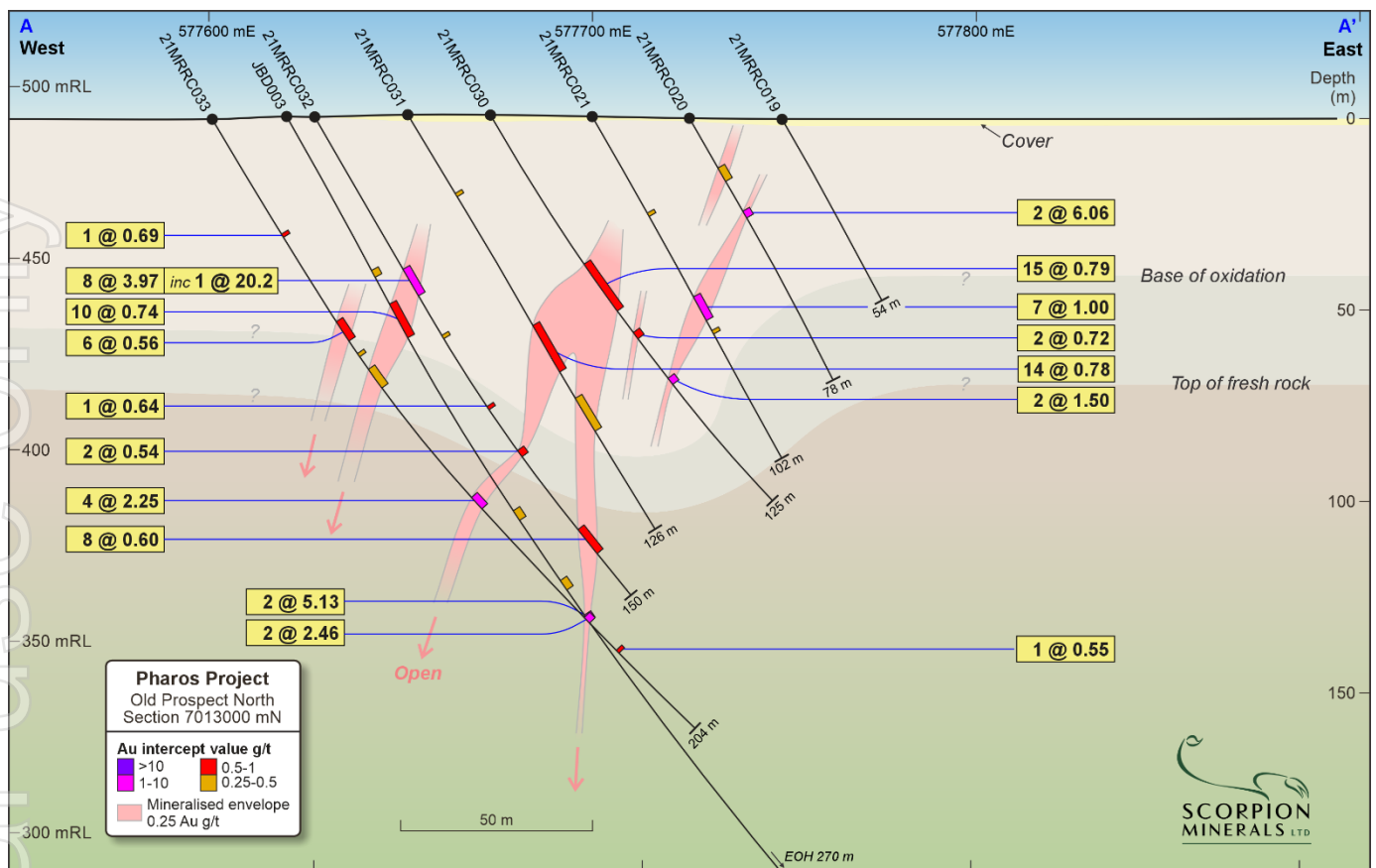
Figure 5: Old Prospect North Section A – A'
