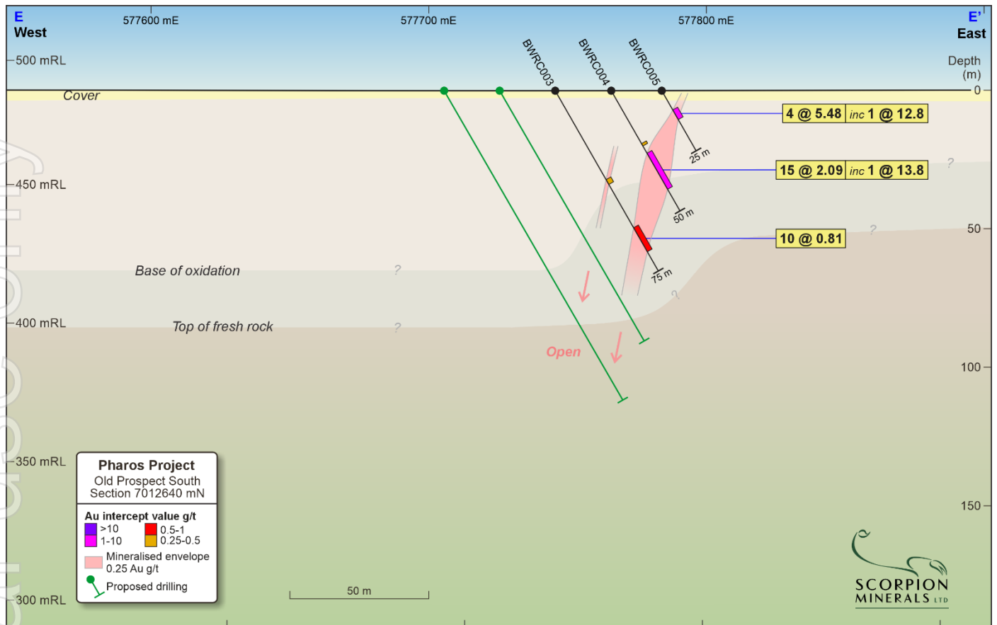
Figure 9: Old Prospect South Section E – E'
