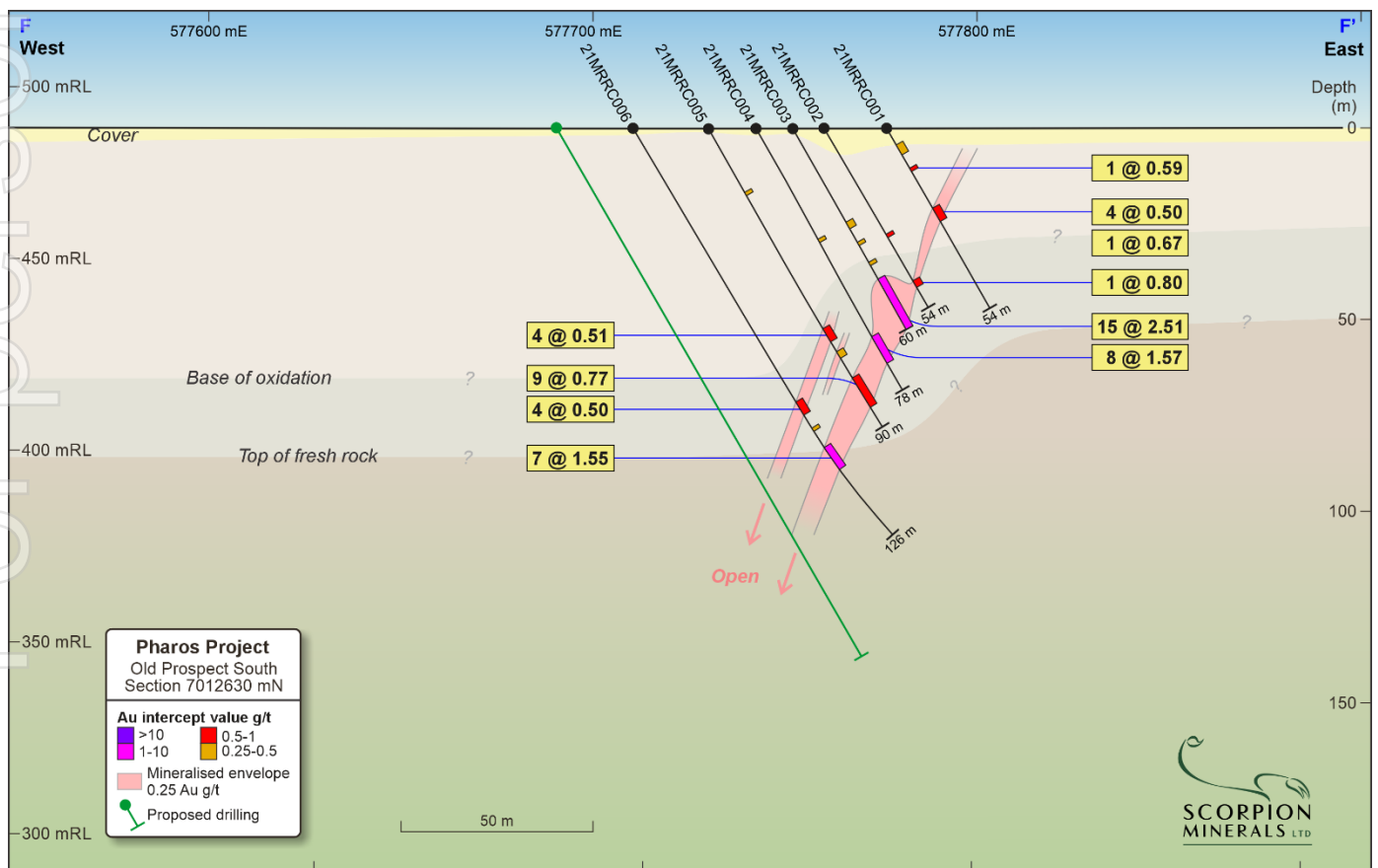
Figure 10: Old Prospect South Section F – F'
