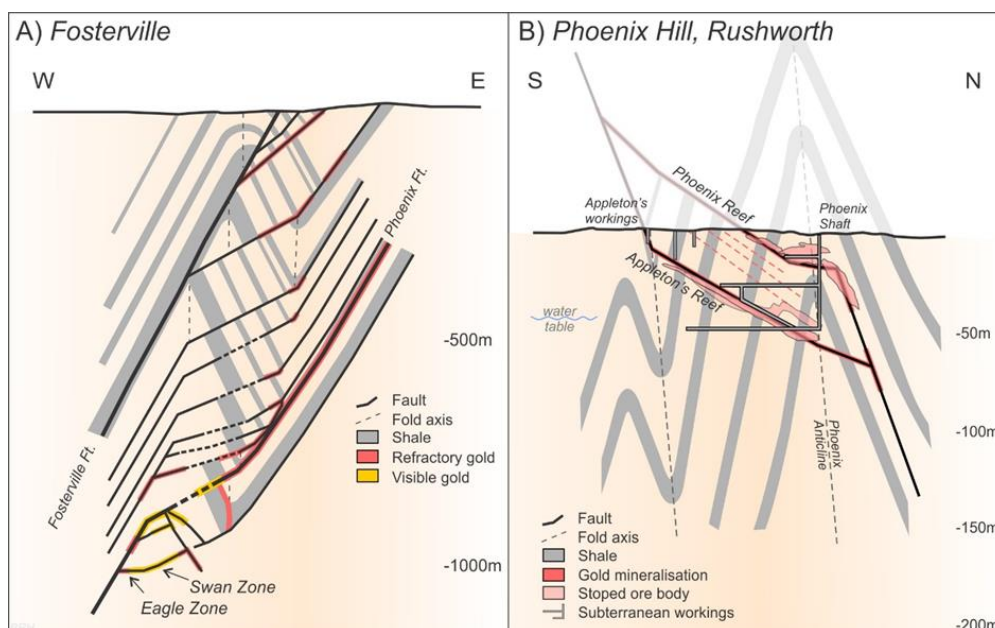
Figure 4: Phoenix Hill cross-section compiled from geological mapping completed by Jones & Turnbull (2014) and Boucher (2016). Figure modified from Dart Mining ASX November 2020.
