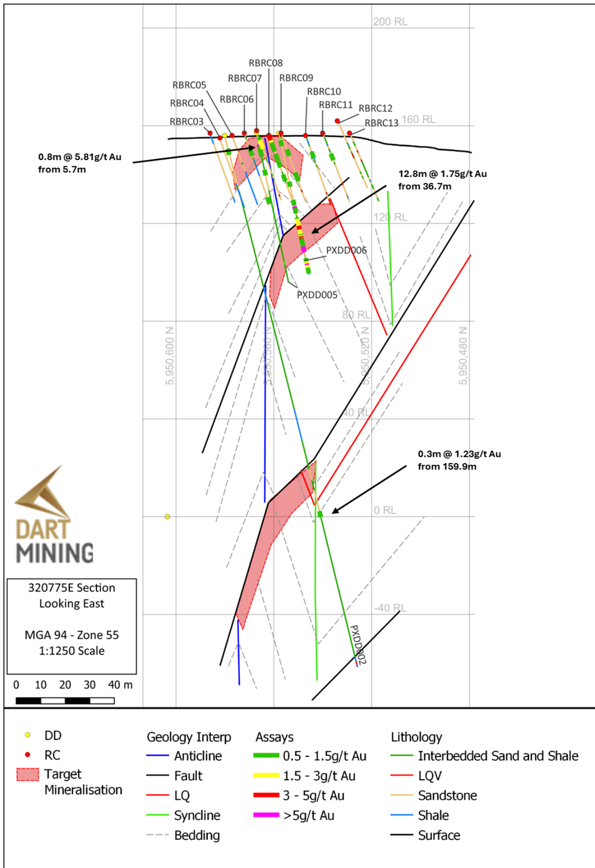
Figure 2: 320775E section showing PXDD002, PXDD005 & PXDD006 with geological interpretation highlighting fold closure offset and prospective zones of mineralisation.
