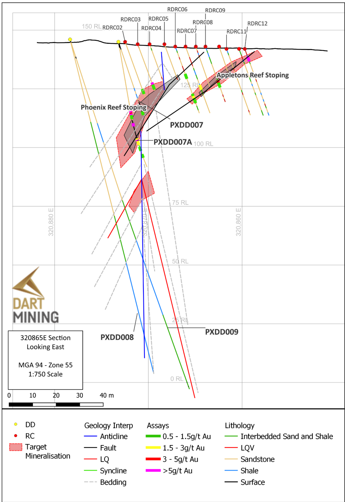
Figure 3: 320865E section showing PXDD007, PXDD007A, PXDD008 & PXDD009 with geological interpretation highlighting fold closure offset and prospective zones of mineralisation.
