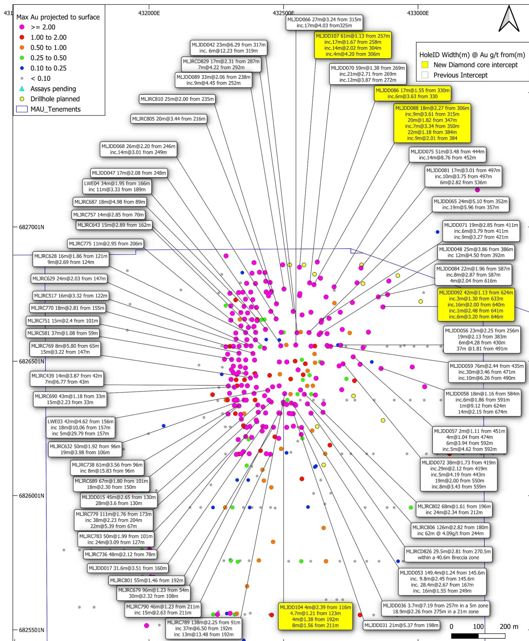
Figure 2. The Lady Julie North 4 deposit has numerous significant thick intersections from the latest drill programme (yellow large rectangular label) and previous drilling (white label) and recently completed drill holes with assay pending in a green label, with maximum gold projected to surface and planned deeper drillholes (in yellow).
