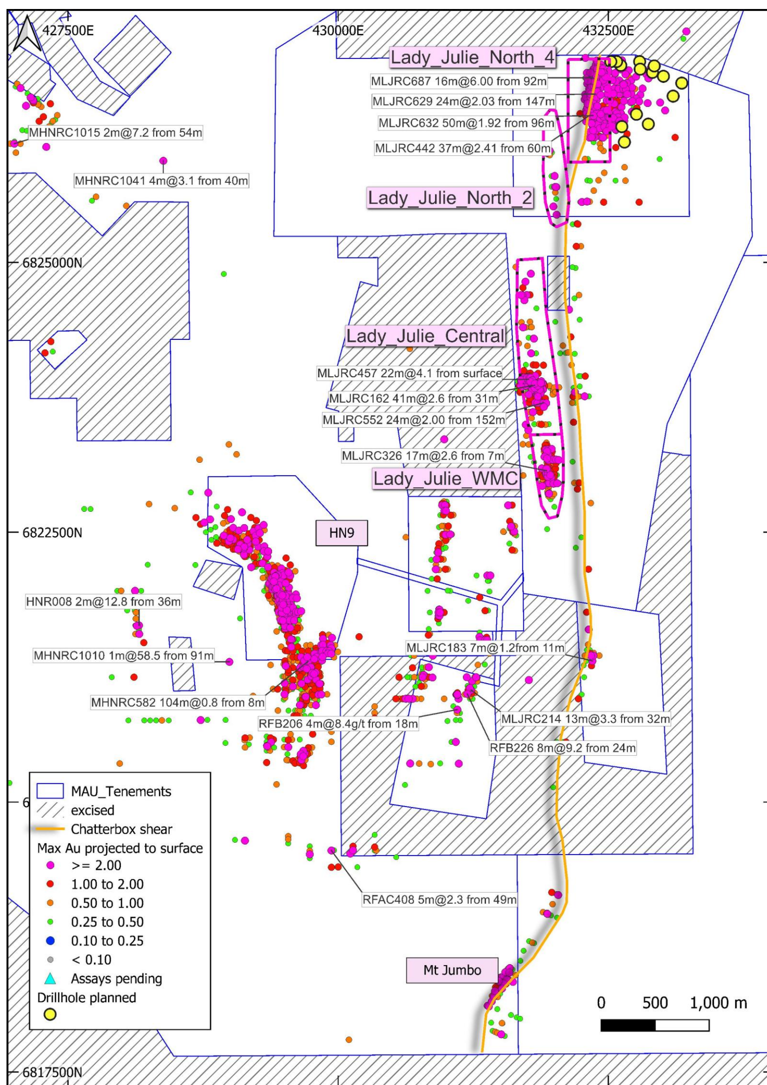
Figure 3. Gold intersection overview covering the Lady Julie North4, Lady Julie Central, Lady Julie WMC, HN9 and Mt Jumbo Projects showing some highlighted intersections (white label), significant historical and Magnetic intercepts (maximum Au projected to surface), planned holes in yellow and highlighted Chatterbox shear extending south from the Lady Julie North 4 Deposit.
