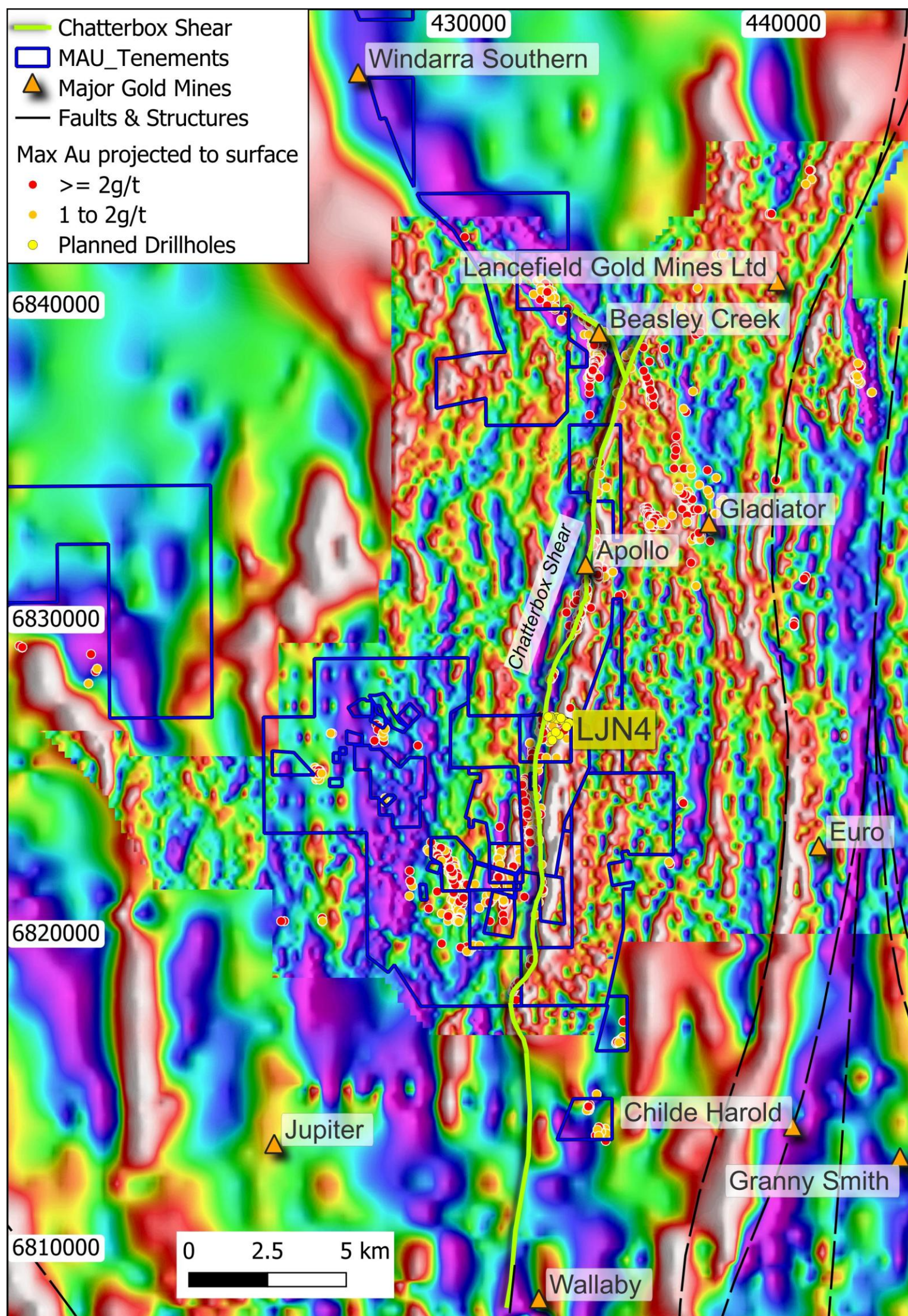
Figure 4. The Lady Julie North 4 Chatterbox Interpreted Shear shown on a Gravity image with major gold deposits
