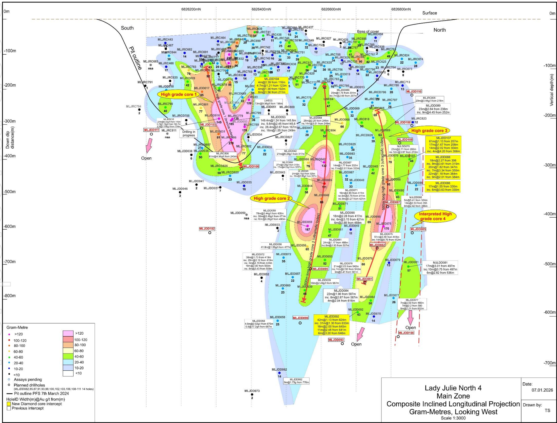
Figure 1. Composite Inclined longitudinal projection of the main lode in LJN4 in gram-metres. Highlighting continuous mineralisation over the whole 750m strike length. Four high grade core zones have been defined. The southern High-Grade Core Zone 1 is 300 x 200m in size and is associated with multiple silica pyrite and breccia lodes. High-grade Core zone 2 is 150m x 600m and is associated with altered silicified and fuchsite ultramafic lodes. HGC3 is 150m x 600m and has similar alteration as HGC2. High-Grade Core 4 is 100m x 500m and has similar alteration as HGC3 and remains open at depth and is currently being tested with further extension holes MLJDD085, MLJDD100, MLJDD108-110.
