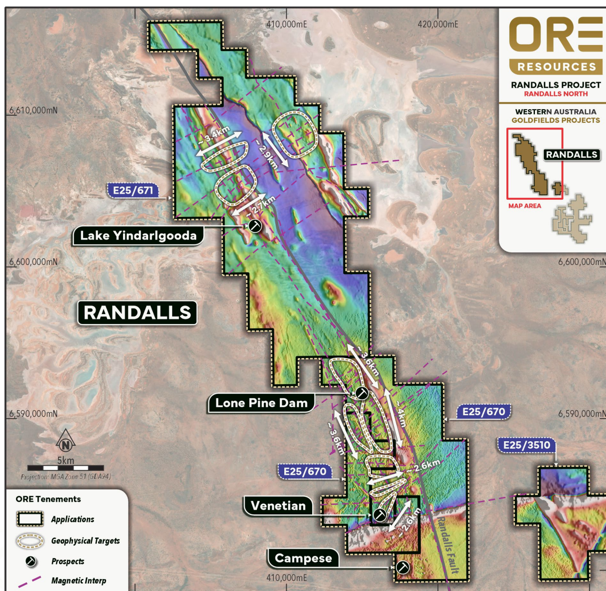
Figure 1: Randalls North geophysical overview and key targets
