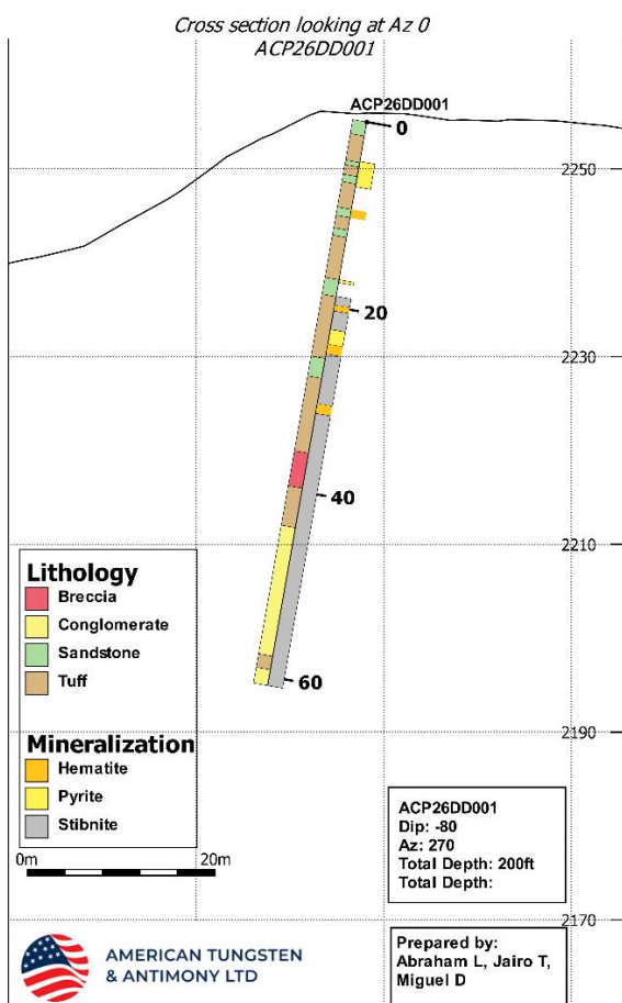
Figure 2 – Schematic representation of the lithology and mineralisation along a hole trace (in metres), with similar information, including visual estimates of the stibnite content, presented on a striplog (in feet).
