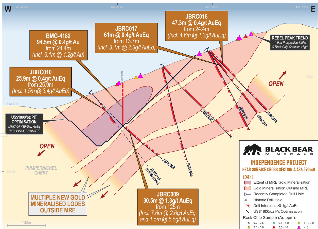
Figure 3: Cross section through the near-surface mineralisation at North Hill, displaying recently received assay results outside the MRE 4 .
