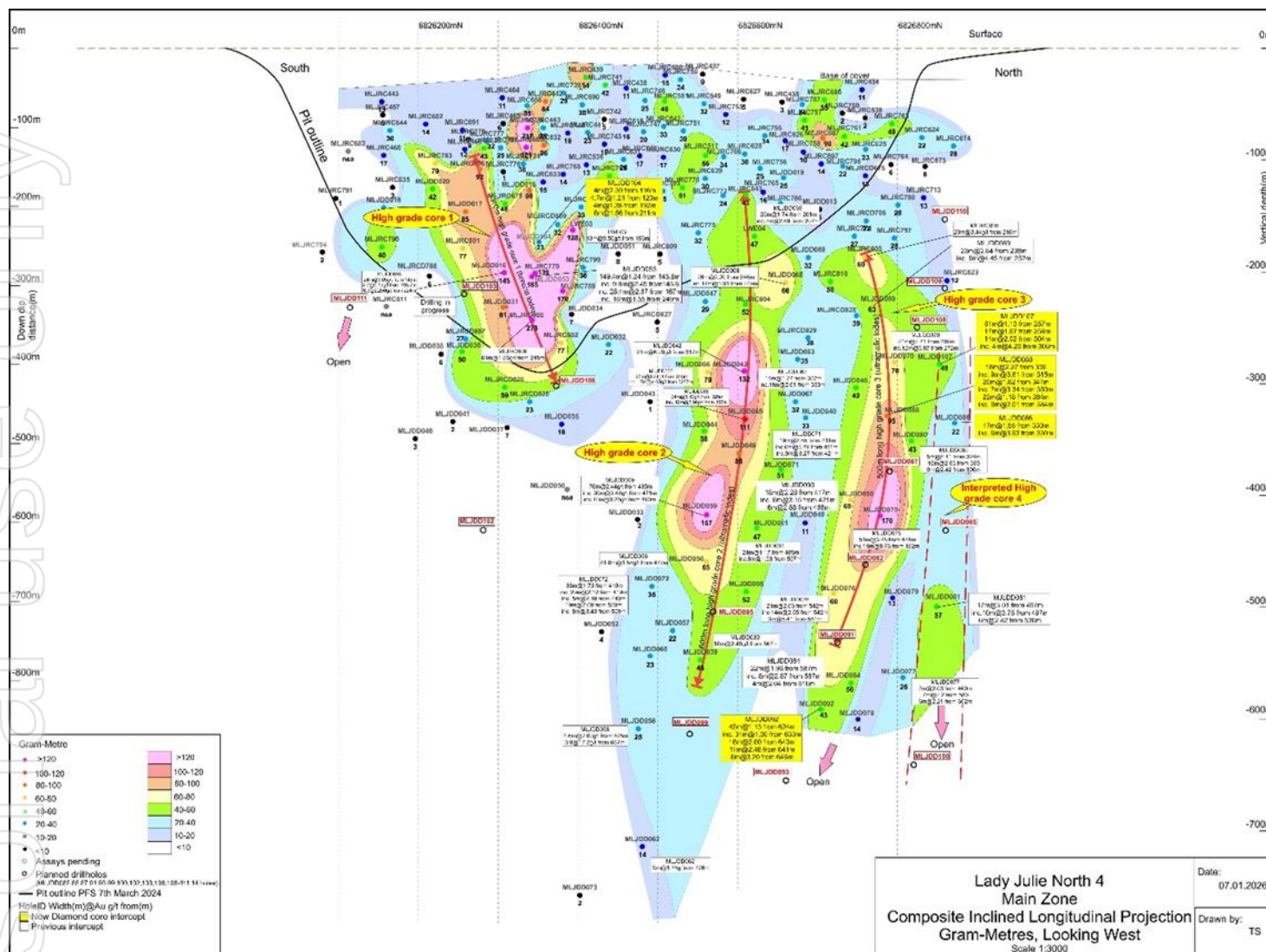
Figure 2. Composite Inclined longitudinal projection of the main lode in LJV4 in gram-metres. Highlighting continuous mineralisation over the whole 750m strike length. Four high grade core zones have been defined. The southern High-Grade Core Zone 1 is 300 x 200m in size and is associated with multiple silica pyrite and breccia lodes. High-grade Core zone 2 is 150m x 600m and is associated with altered silicified and fuchsite ultramafic lodes. HGC3 is 150m x 600m and has similar alteration as HGC2. High-Grade Core 4 is 100m x 500m and has similar alteration as HGC3 and remains open at depth and is currently being tested with further extension holes MLJDD085, MLJDD100, MLJDD108-110.
