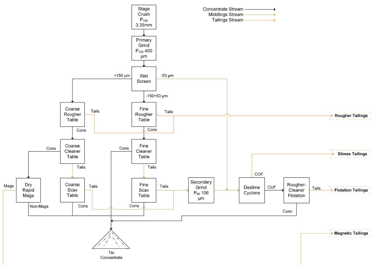
Figure 2. Block Flow Diagram – Test work Flowsheet
