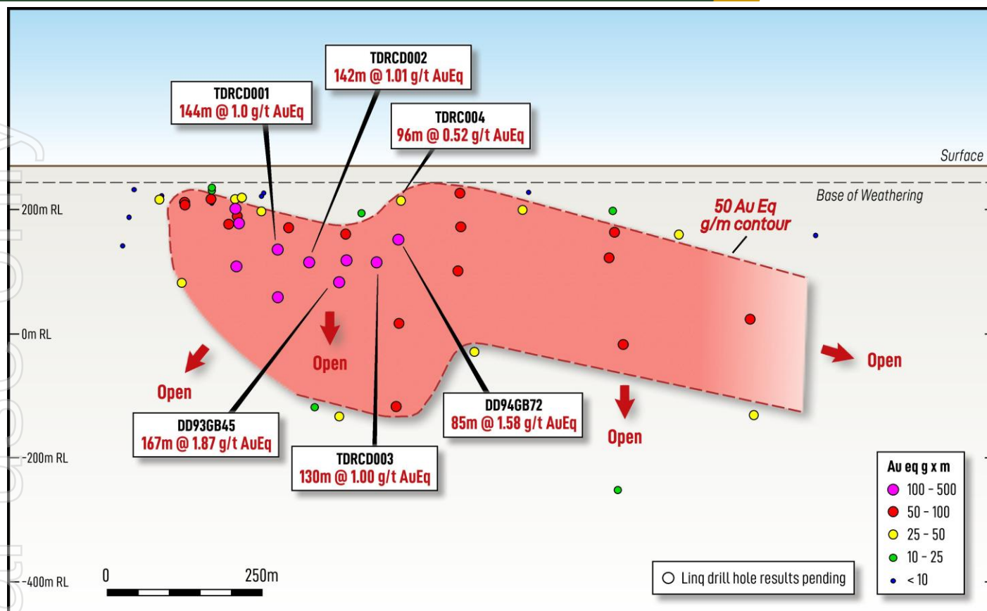
Figure 3: Dam long section illustrating the results from Linq holes TDRCD001, TDRCD002, TDRCD003 & TDRCD004 along with historical holes DD93GB45 & DD94GB72.
