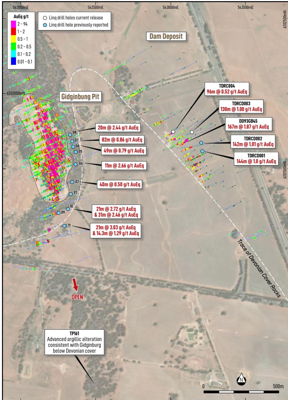
Figure 1: Gidginbung/ Dam plan image illustrating the location of drilling results.
