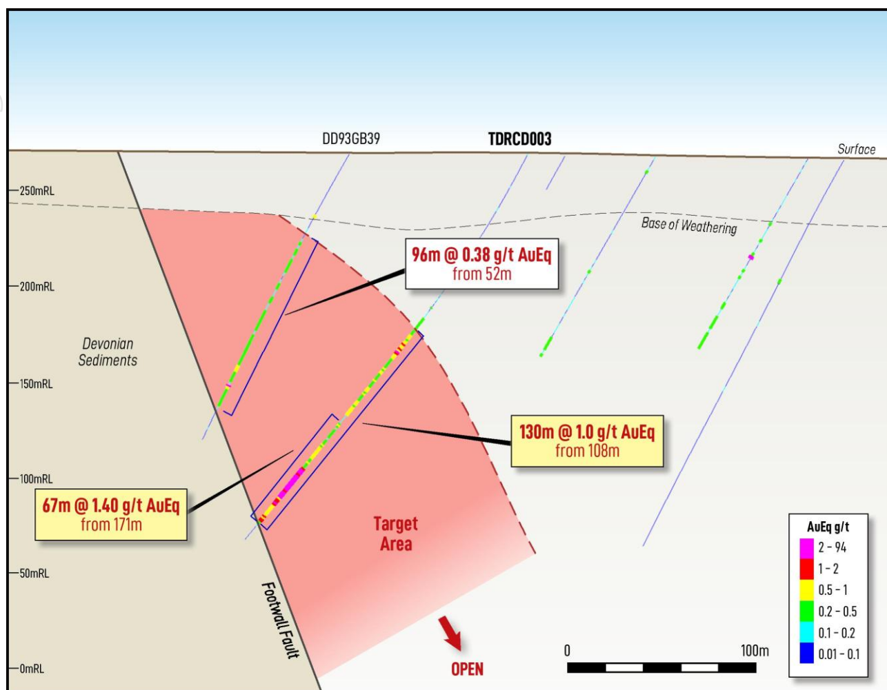
Figure 2: Dam cross section illustrating the results from hole TDRCD003 (local northing 9040N).
