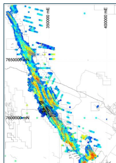
FIGURE 5 – Detailed airborne magnetics
