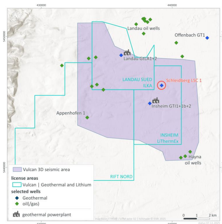
Figure 1: Location map for the Schleidberg LSC-1 well.
