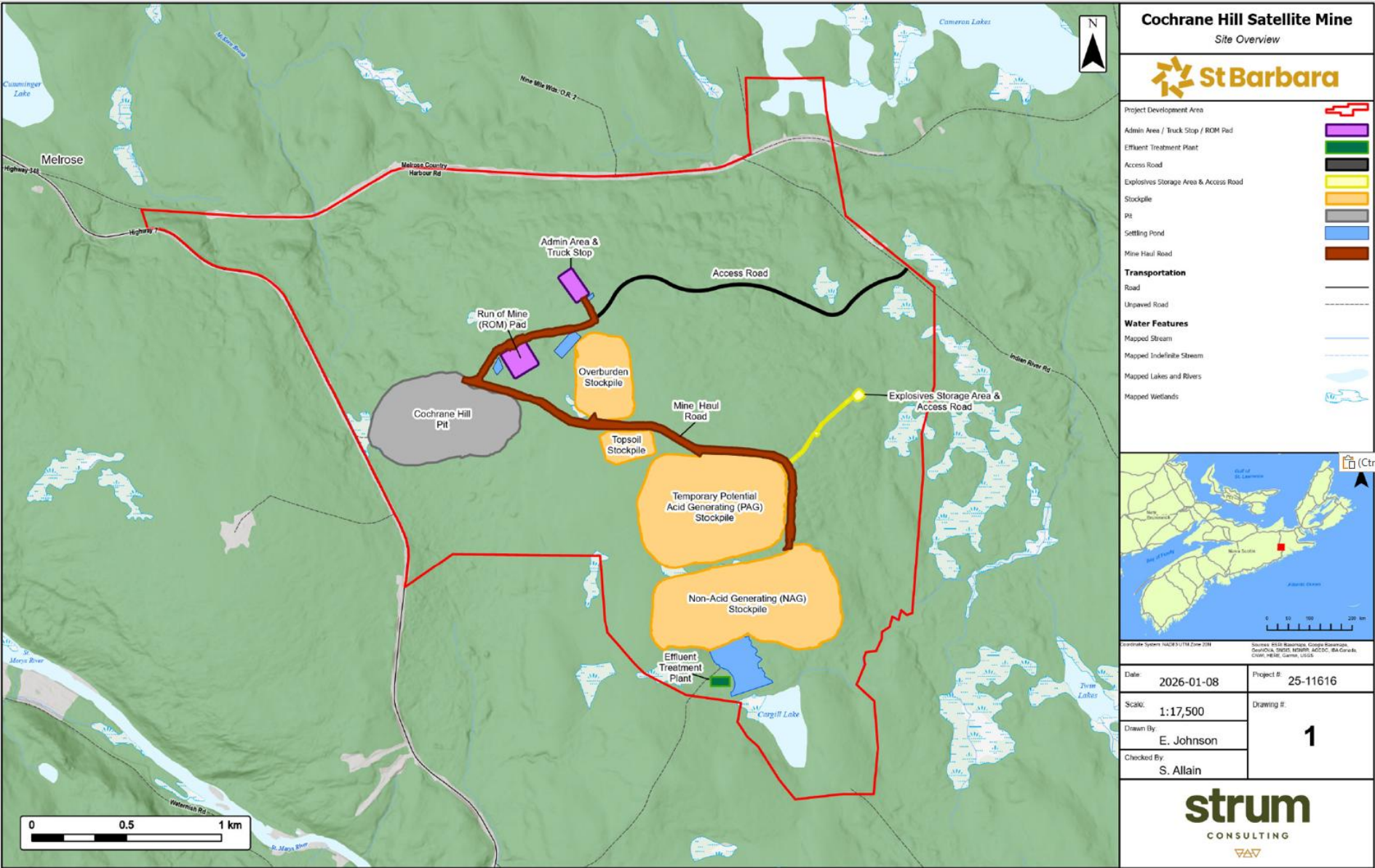
Figure 3: Cochrane Hill Satellite Mine Layout
