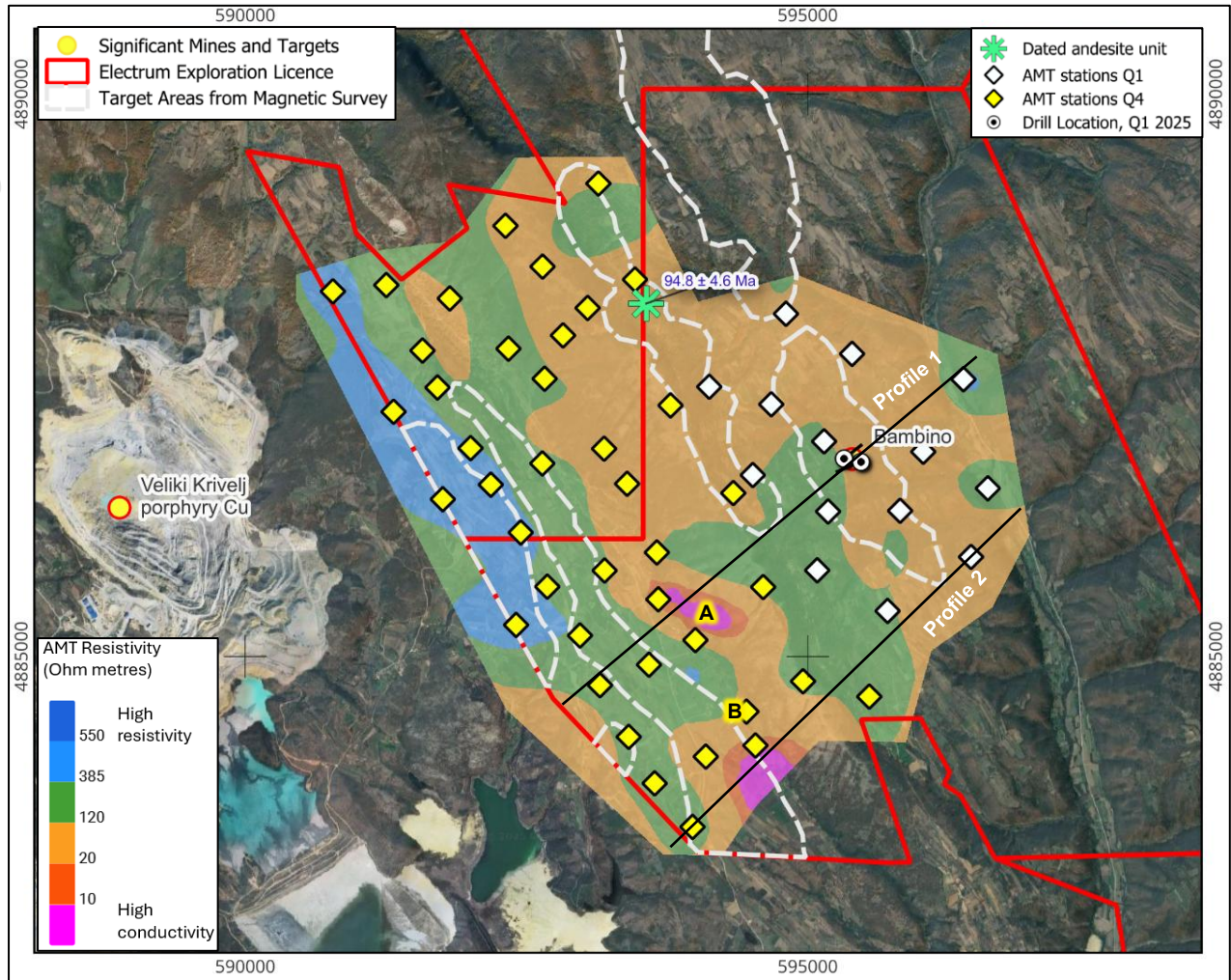
Figure 3: - Horizontal slice through the modelled AMT resistivity at 80m below reference-level (approximately 250m to 550m below surface level in the survey area). High conductivity areas marked as "A" & "B" (WGS84 z34N)
