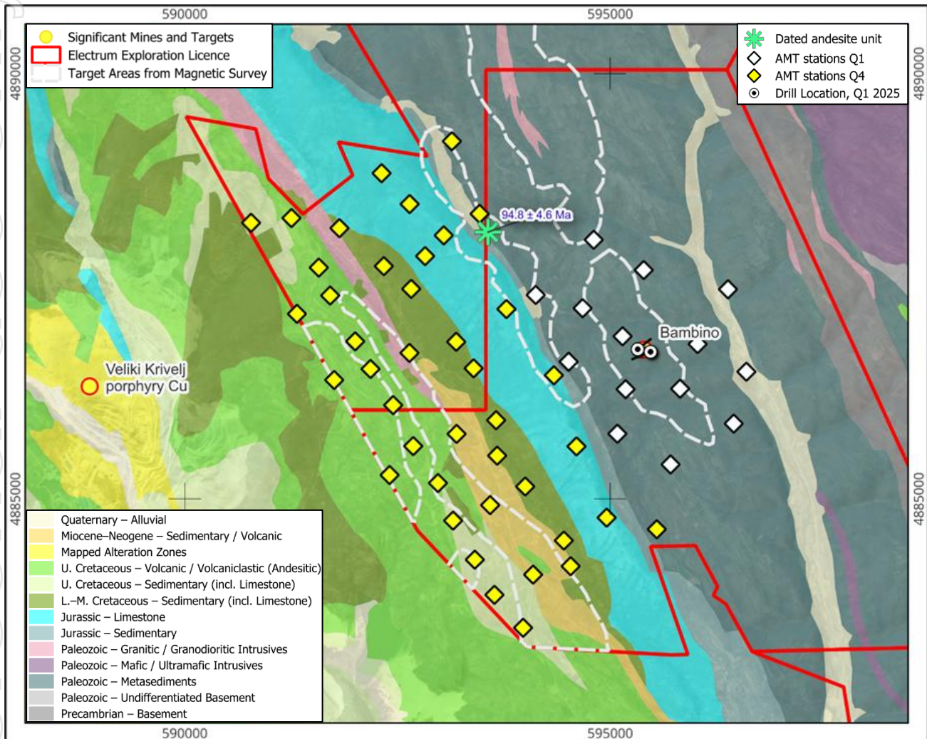
Figure 2: - AMT stations for both surveys in 2025 overlain on district geology with targets identified from previous ground magnetic survey (WGS84 z34N)
