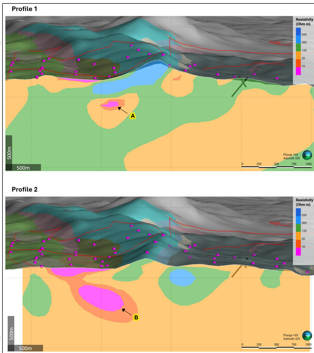
Figure 4: - Vertical slices through the modelled AMT resistivity along Profiles 1 and 2 (refer Figure 3). Target areas of high conductivity marked as "A" and "B". Vertical and horizontal scales are equal; view angle is slightly downwards and looking to the NW.
