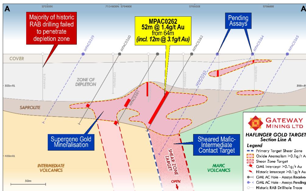
Figure 2: Cross Section A extensive supergene mineralisation above the target sheared mafic-intermediate contact.
