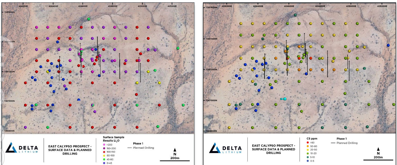
Figure 8: Plan Views to East Calypso with surface data showing lithium & caesium anomalism
