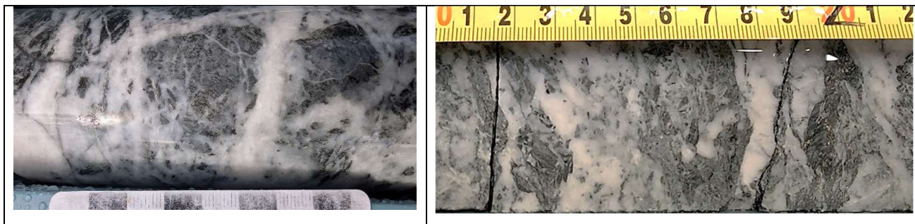
Figure 1a NSD057 - stock-worked, silicified breccia
