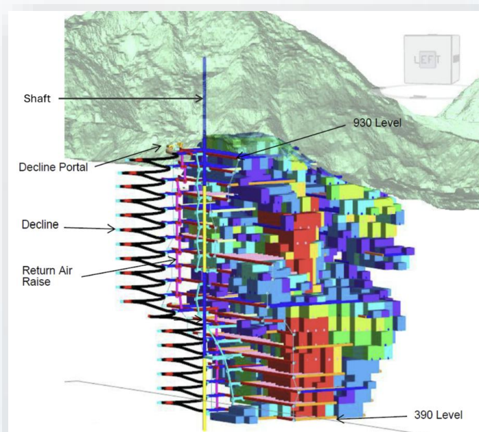
Figure 2: Image of stoping and decline development
