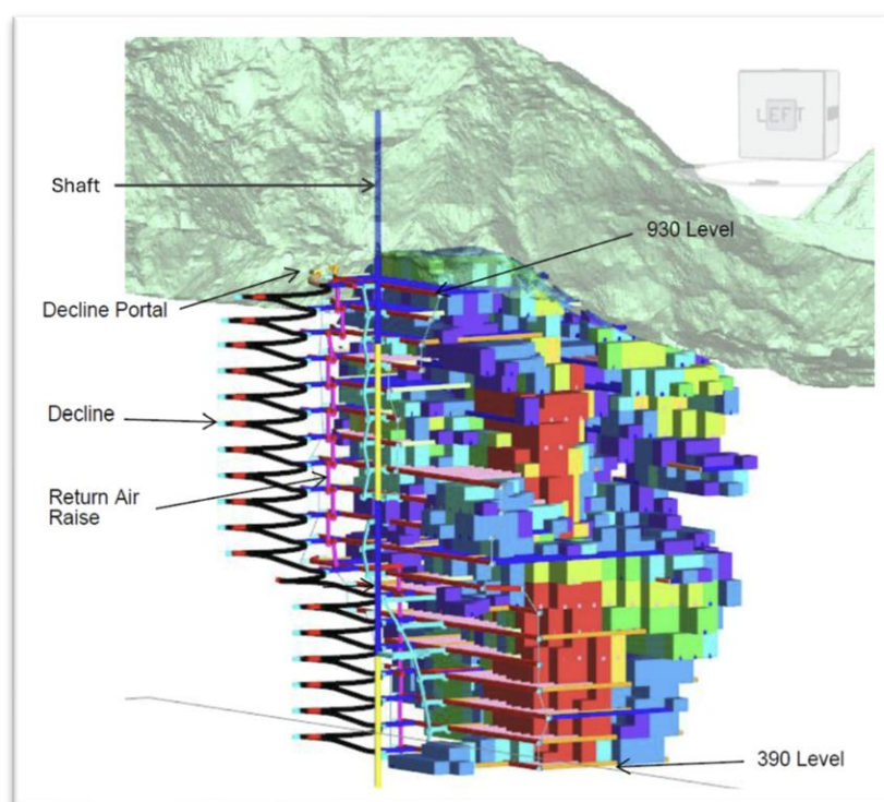
Figure 2. Image of stoping and decline development.
