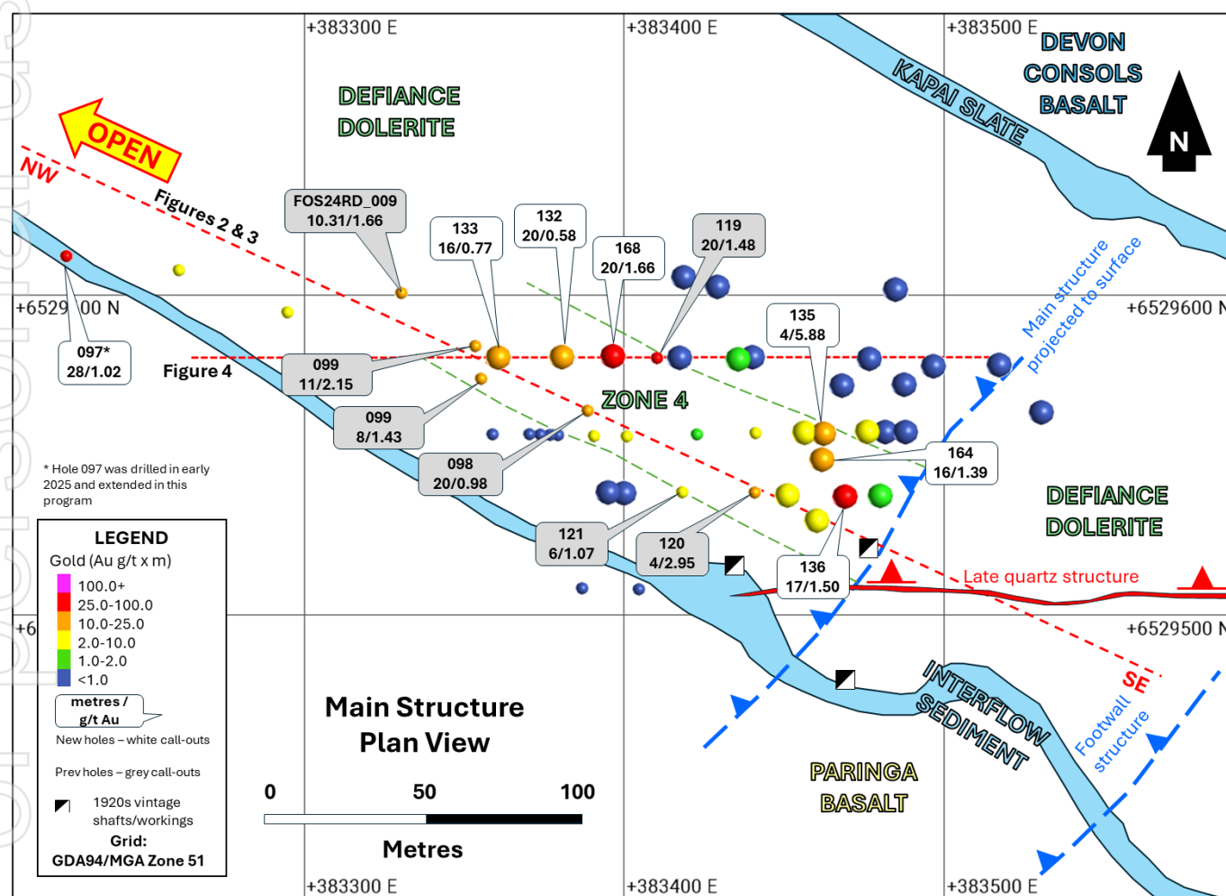
Figure 1: Plan view of the Hustler Prospect showing today's results (white call-outs and/or large circles), previous results (small circles and/or grey call-outs) and location of the long section in Figures 2 & 3 and the cross section in Figure 4 .
