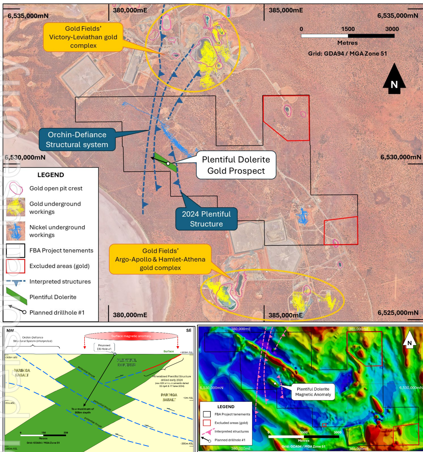
Figure 5: Compilation of views, plan and sectional, view of the FBA showing the Orchin-Defiance structural system and the Plentiful Dolerite prospect over an aerial photo depicting key local infrastructure and past producing gold mines on adjacent Gold Fields' ground.
