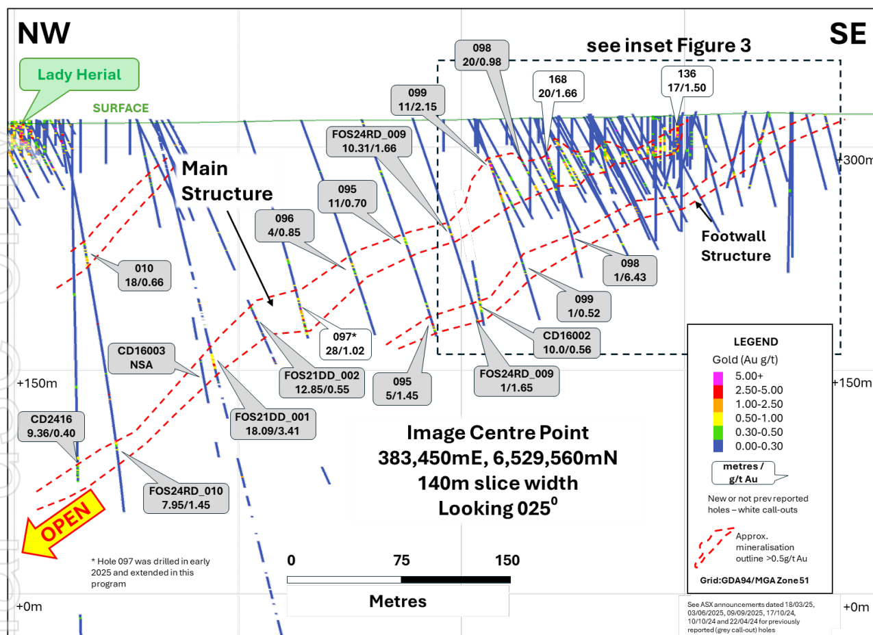
Figure 2: Long section view of the Hustler Prospect showing today's and prior results (grey call-outs) and inset of Figure 3.
