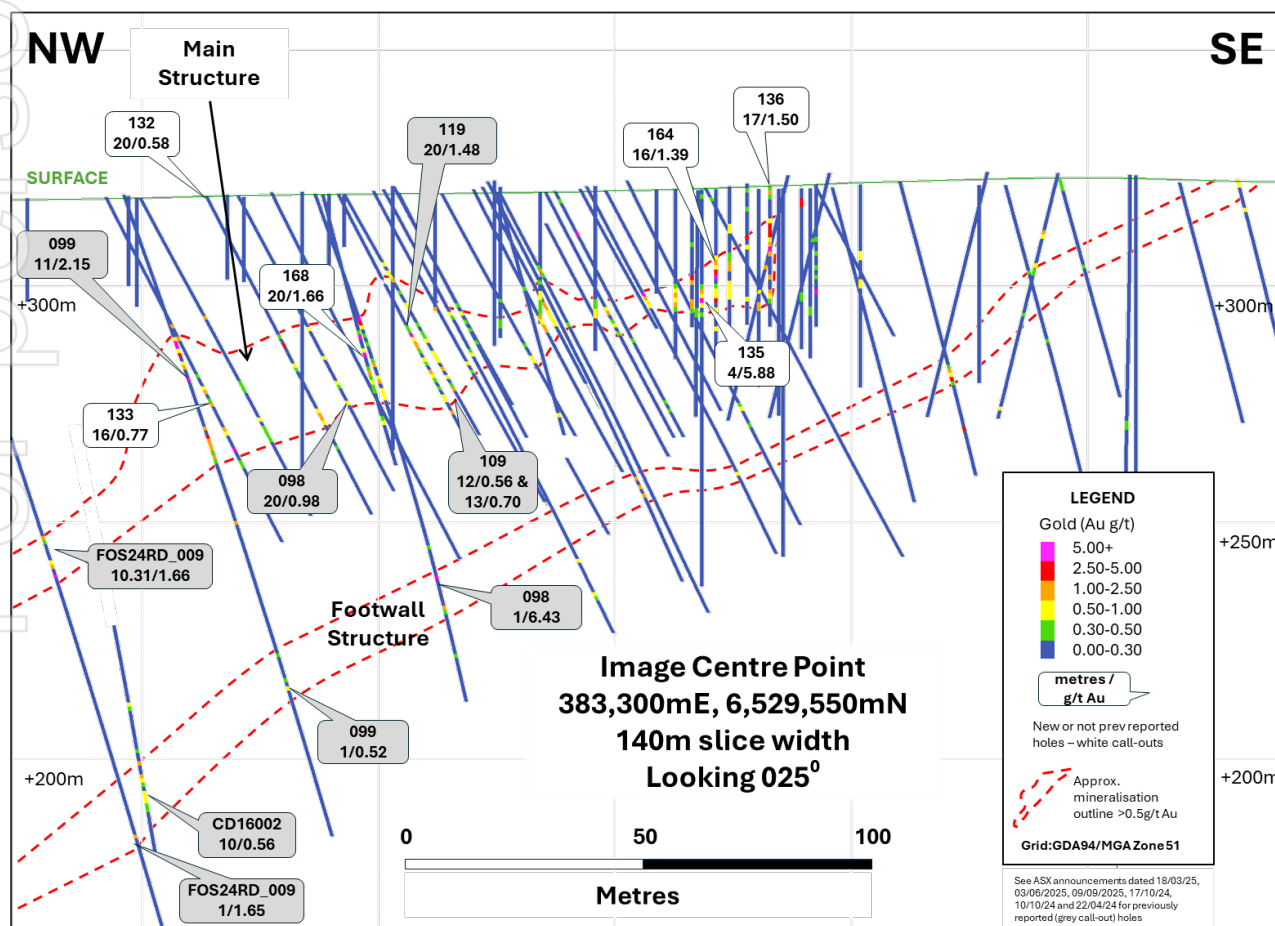
Figure 3: Inset view from Figure 2, long section view of the Hustler Prospect showing today's and prior results (grey call-outs).
