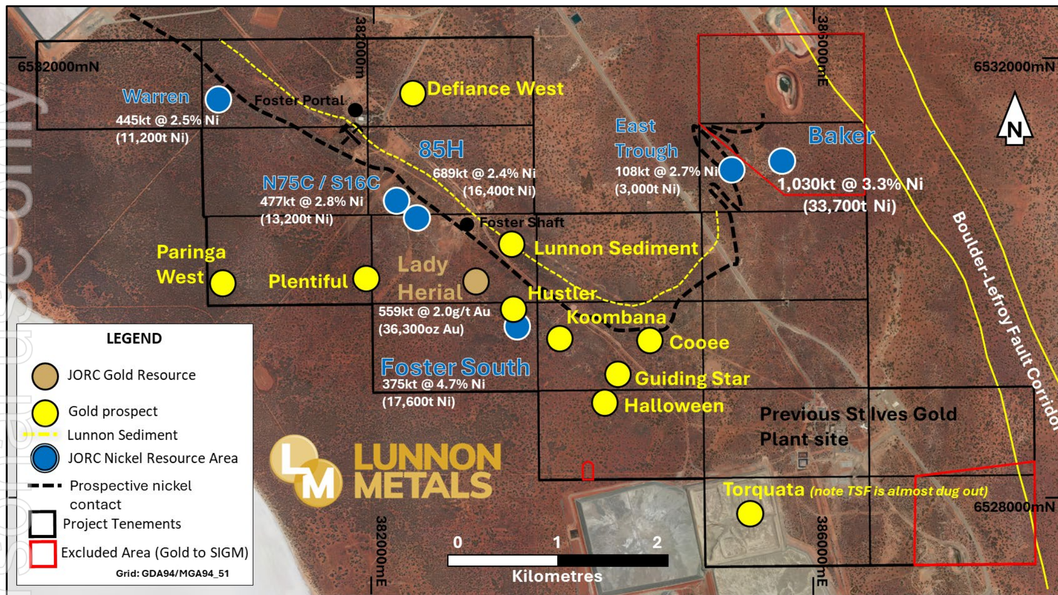
Figure 6: Foster-Baker Project Area showing location of the Plentiful and Hustler gold prospects along with other select high-ranking gold prospects, and gold & nickel Mineral Resource 2 positions.
