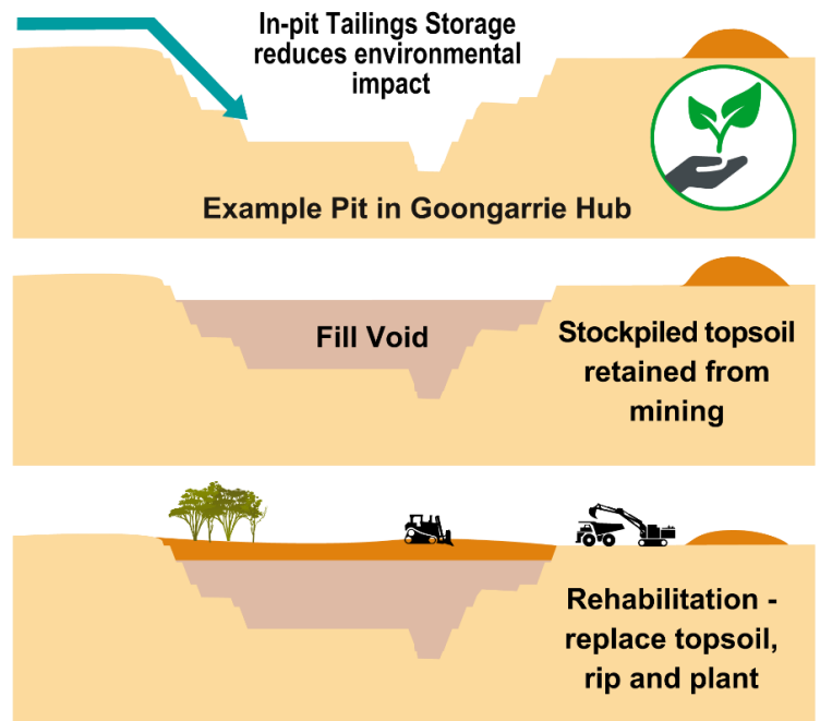
Figure 4: Planned Goongarrie Hub in-pit tails disposal and rehabilitation strategy.
