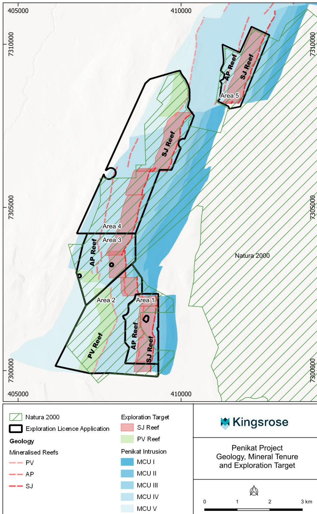
Figure 2: Kingsrose mineral tenure and geology of the Penikat Project, Finland.
