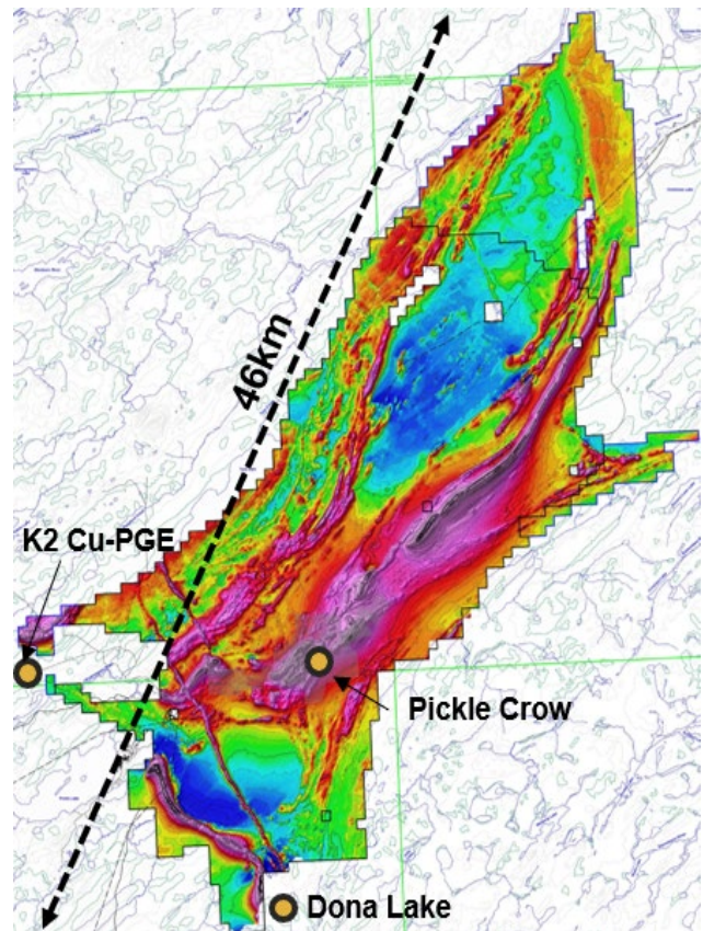
Figure 7: Helicopter magnetics.
