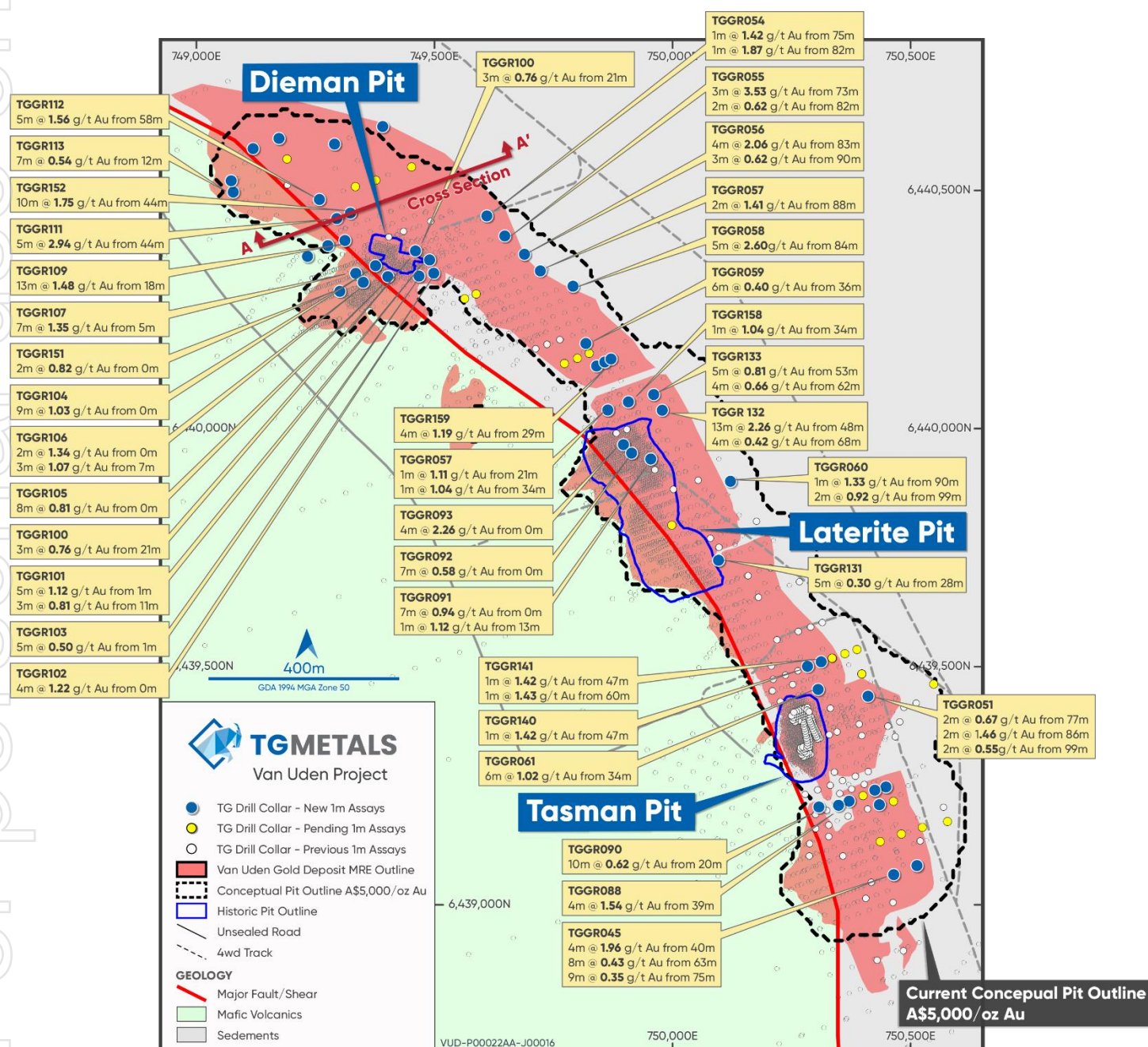
Figure 1 – New Resource Drilling Collars Showing Select Intercept Highlights (New Results in Yellow) and Pending Assay Drillholes marked yellow collars
