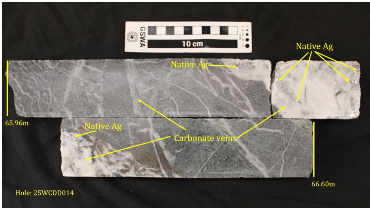
Photo 3: Photograph of cut half HQ3 drill core (25WCDD014) from 65.96m to 66.60m showing 1% visually estimated, 2mm to 3mm long native silver grains hosted in and adjacent to 1cm to 10cm thick carbonate veins in an ultramafic host rock.
