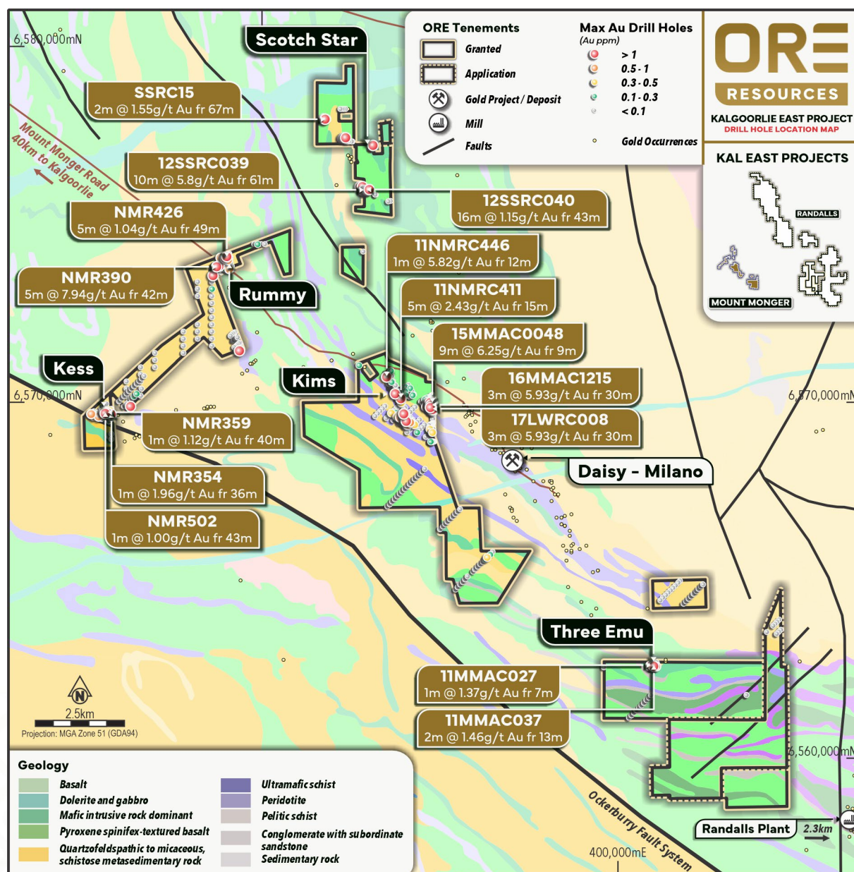
Figure 2: Project plan view with drill hole max down hole gold
