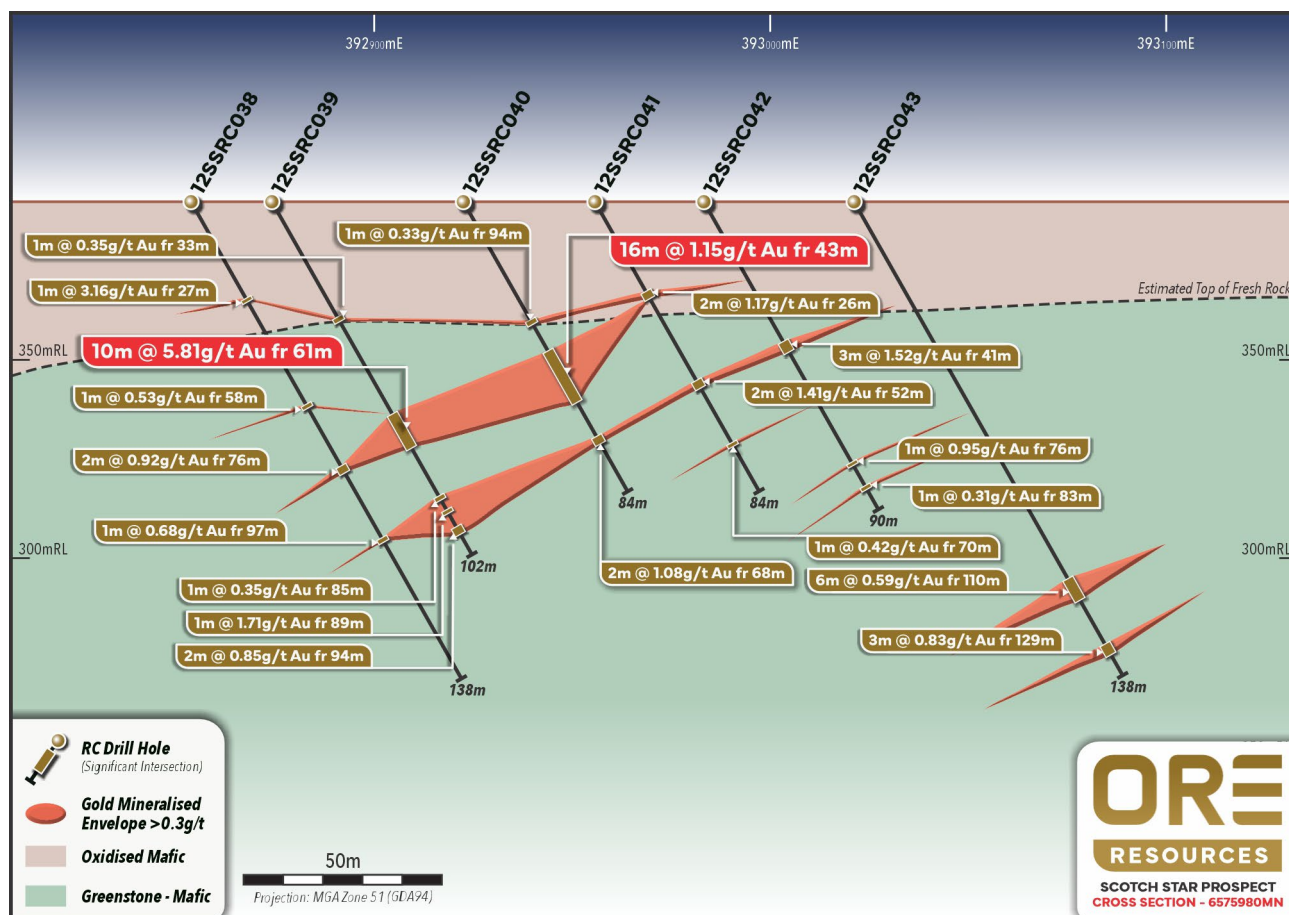
Figure 3: Cross-Section – Scotch Star
