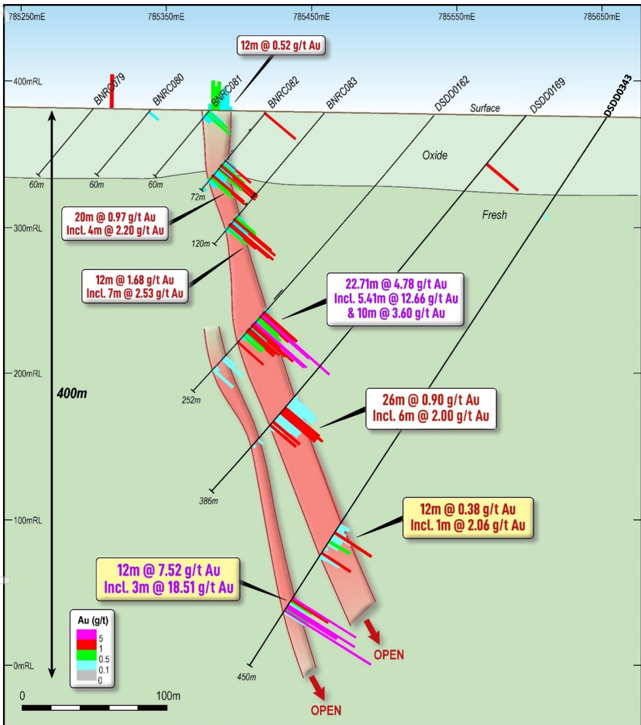
Figure 7: Cross Section looking north (+/-25m) showing new drill results (yellow) for BDT3 11
