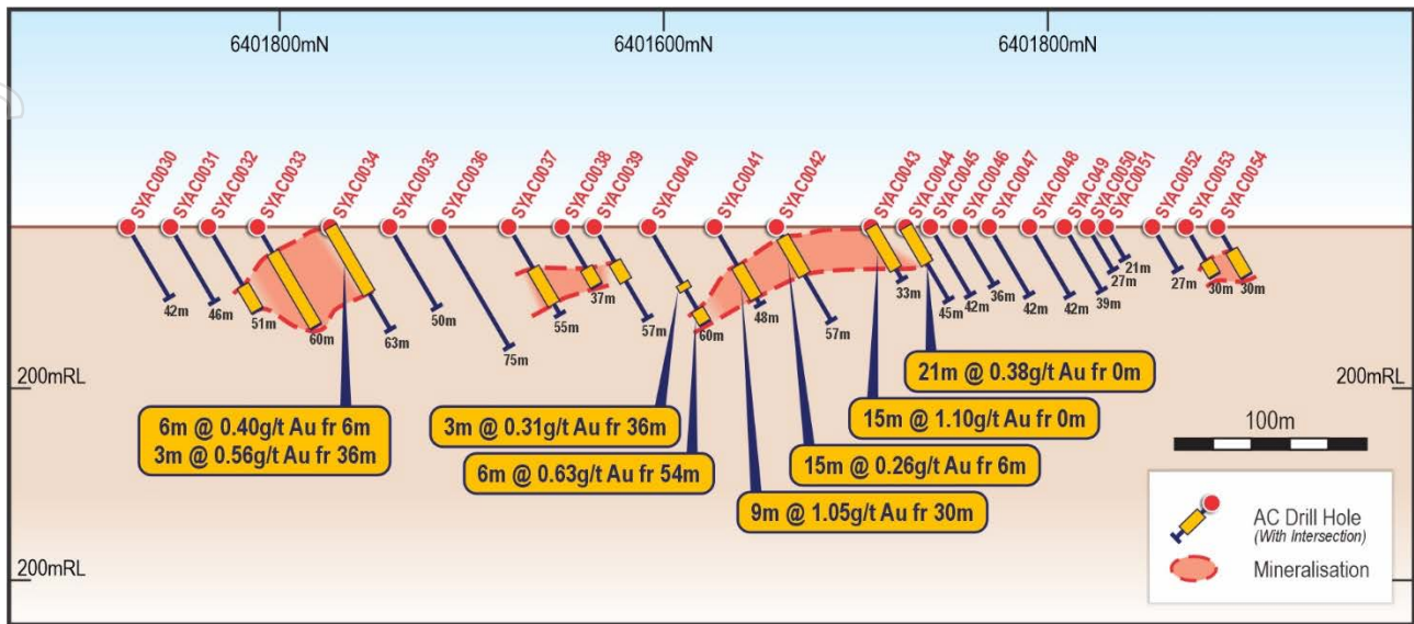
Figure 4. Sheepyard Prospect western line of AC drilling - cross section 479050E looking east. A zone of highergrade gold mineralisation, approximately 60m wide at surface, is indicated by the near-surface intersections in holes SYAC00040 to SYAC00044 within a broad zone of low-grade gold mineralisation. High-grade intersections include 15m at 1.10g/t Au from surface in SYAC00043 and 9m at 1.05g/t Au from 30m in SYAC00041 are highlighted. Assaying is by 3m composite sample. True width of mineralisation is not known.
