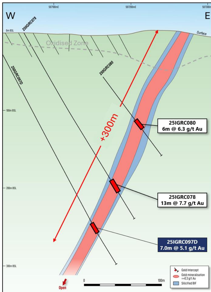
Figure 2: Schematic cross-section of the Vadrians gold deposit showing recent drill intersections (blue box).
