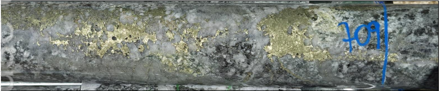
Core photo from DKD039 (709m downhole) showing vein-hosted and disseminated chalcopryite (~3%) and pyrite (~2%) mineralisation in strongly veined tonalite host rock, assay results expected April 2026¹
