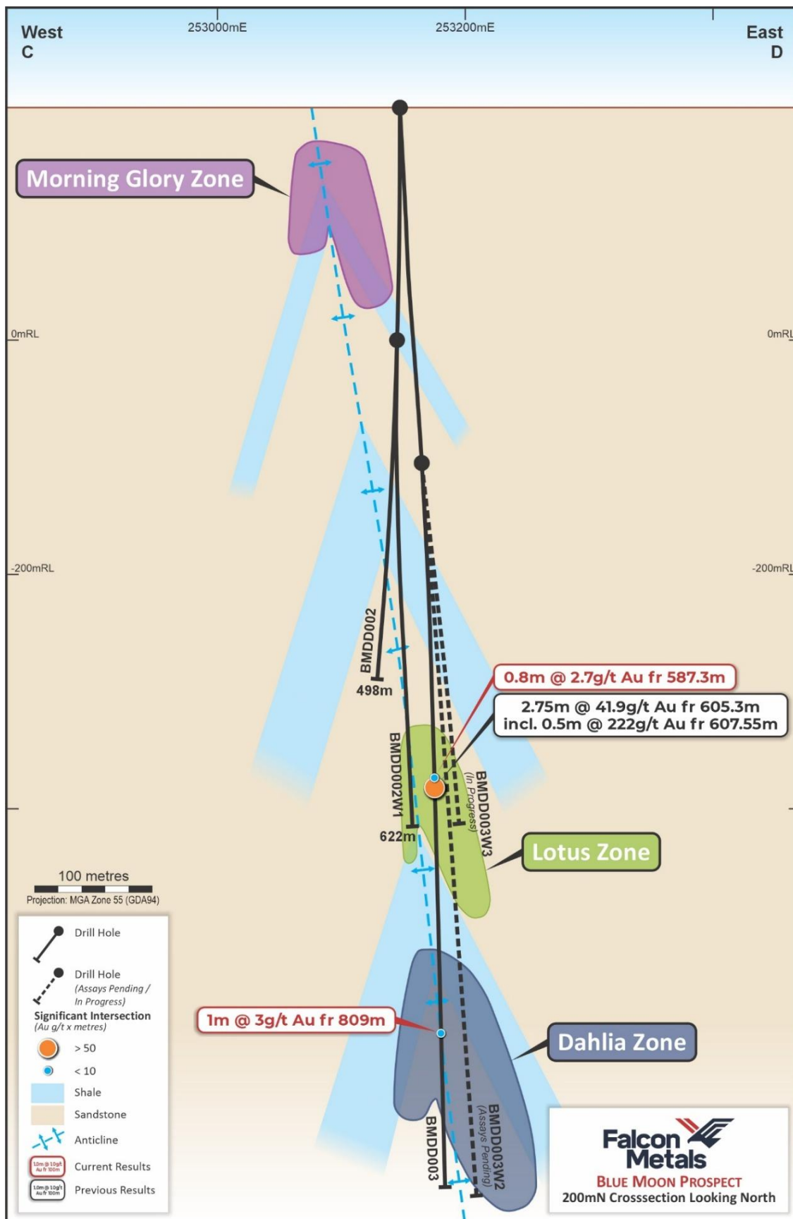
Figure 8 Second Section - schematic cross section of BMDD002 and BMDD003 looking north show the Lotus Zone and Dahlia Zone
