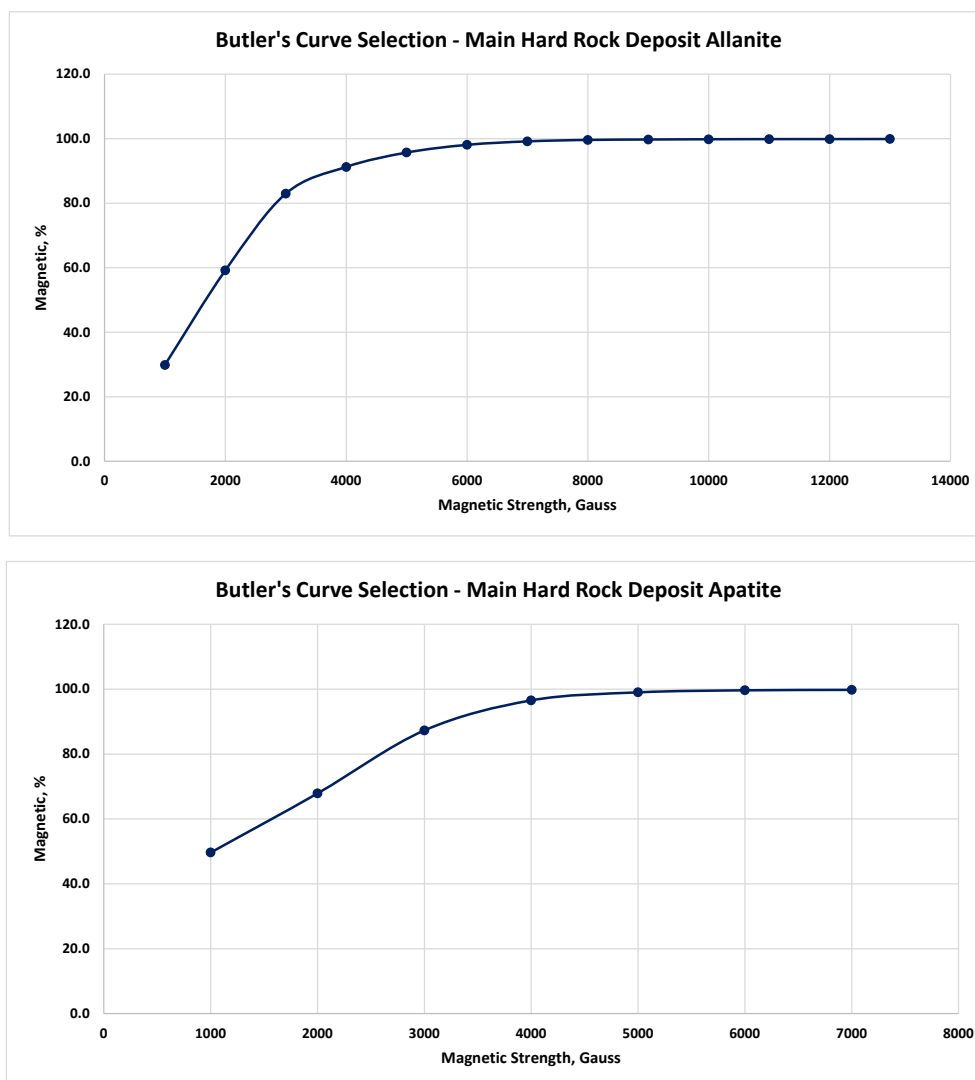
Figure 1 – Magnetic Separation Test Work – Korsnäs Samples
