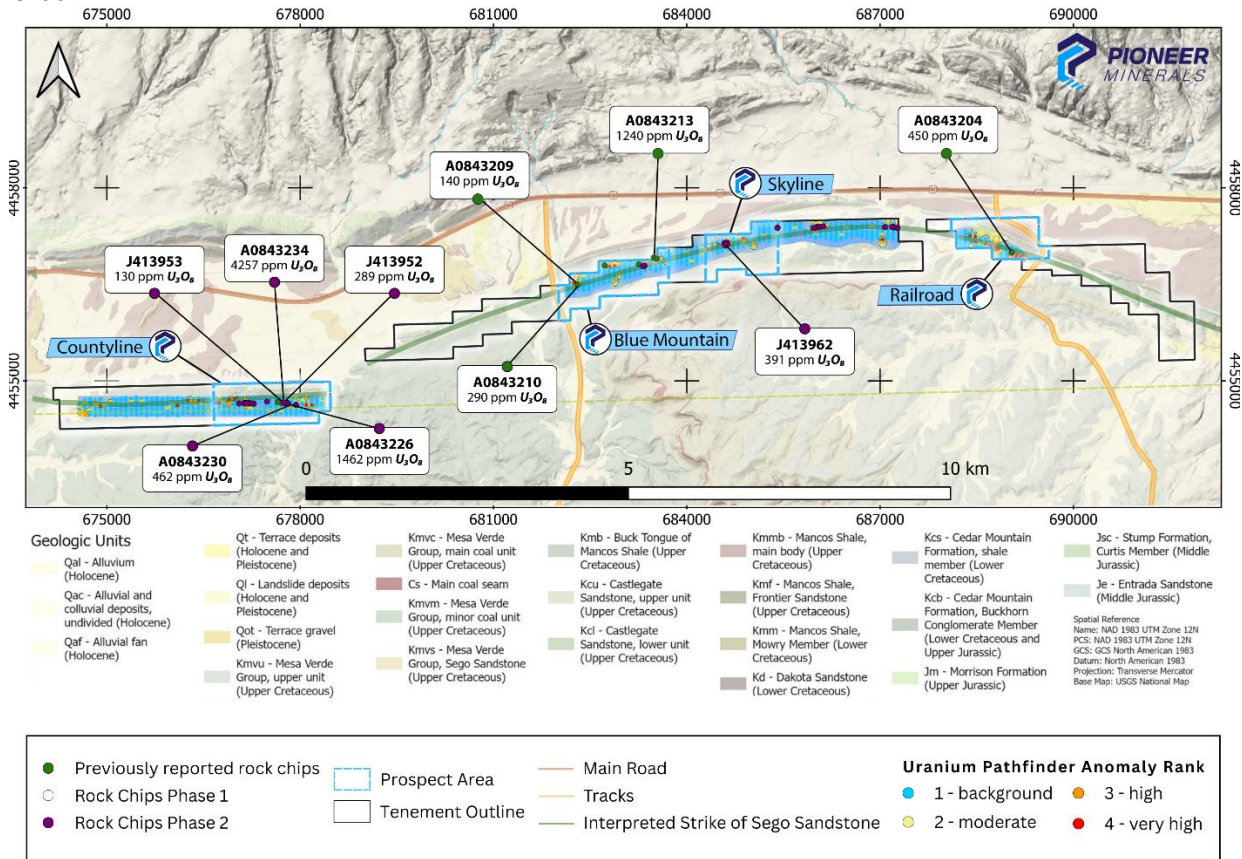
Figure 1: Skull Creek Uranium Project overview showing all rock chip samples results above 100 ppm U_3O_8 and interpreted soil geochemistry results from both phases of soil sampling at Skull Creek. All rock chip samples and soil geochemistry from both phase 1 and 2 are included as appendix A and B.
