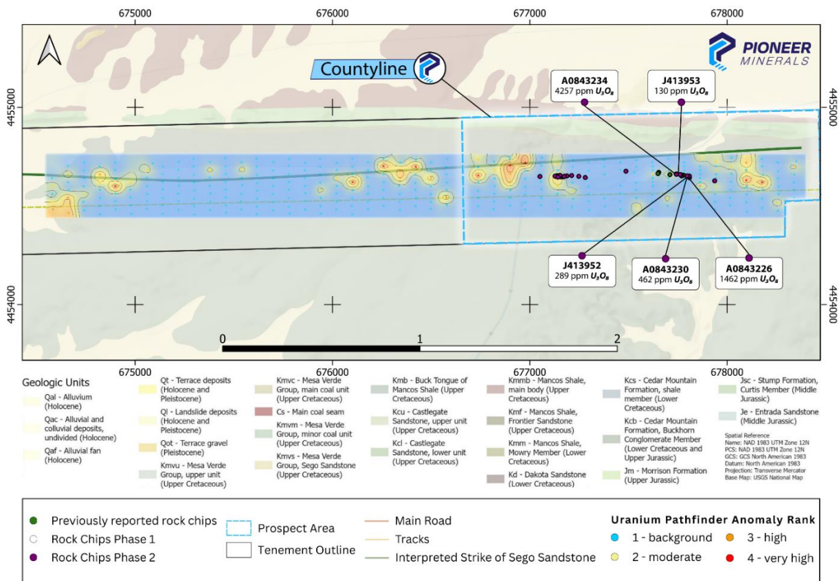
Figure 2: Showing the western portion of the Skull Creek Uranium Project and the Countyline Prospect where high grade rock chips samples returned grades of up to 4257 ppm U_3O_8 and geochemical anomalies in soils extending both to the west and east of outcrop.
