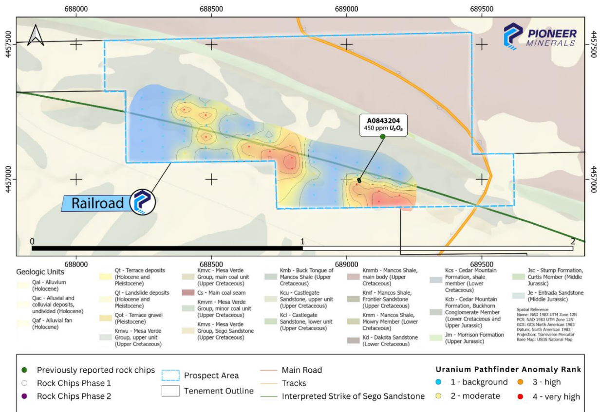
Figure 3: Shows the eastern block and Railroad prospect at the Skull Creek Uranium project where outcrop is limited and contains only one rock chip sample taken during phase 1 of sampling which returned 450 ppm U_3O_8 (ASX: PMM 05/05/2025). Significant pathfinder soil anomalism exists here extending to the east and the west of Sample A0843204 indicating the potential for further mineralisation hidden beneath soils.
