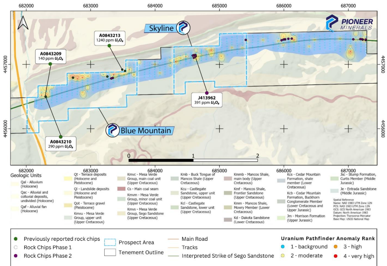
Figure 4: Shows the central block and Skyline and Blue Mountain prospects where previous samples taken during phase 1 exploration returned 1240 ppm U 3 O 8 in sample A0843213 (ASX: PMM 05/05/2025).
